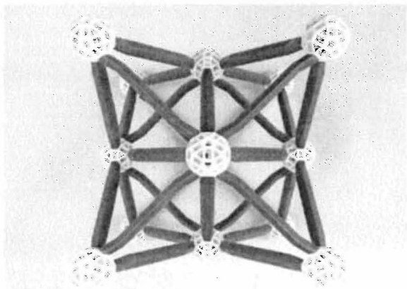
FIG. 43. Face-centered cubic lattice constructed using Zometool. The construction violates four-fold rotation symmetry about the axis perpendicular to the photographic plane and passing through the center node.
