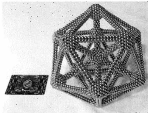
FIG. 19. Photograph of a model of a 13-atom icosahedral cluster made with 3860 Zen Magnets. Such clusters can be formed by neon, argon, krypton, and xenon, and have 12 atoms at the icosahedral vertices and one atom at the center.
