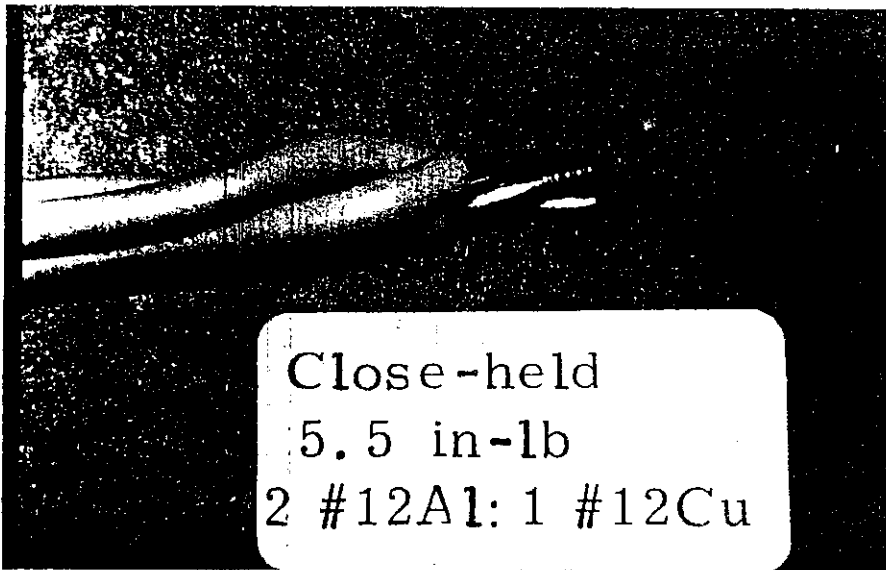
19. THE AMOUNT OF TWISTING TOGETHER OF THE WIRES VARIES SUBSTANTIALLY WITH THE HARDNESS, SIZE(S), AND NUMBER OF WIRES INSTALLED. Inadequate mechanical disturbance results in poor electrical contact at the wire-to-wire interface. THIS IS A FUNDAMENTAL DEFICIENCY OF TWIST-ON CONNECTIONS WITH ALUMINUM WIRE
