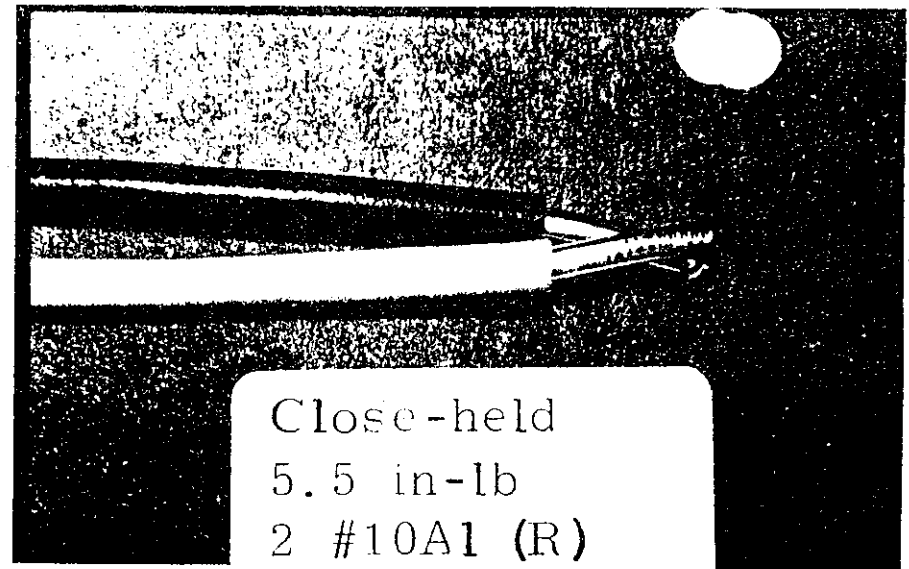
18. CURRENT FLOW IN THE STEEL SPRING occurs due to a fundamental deficiency of this type of connection when made with aluminum wire. There is inadequate metallic contact directly established from wire-to-wire. The insulating oxide on the aluminum is not sufficiently broken up. (Photo: connector removed after splicing.)
