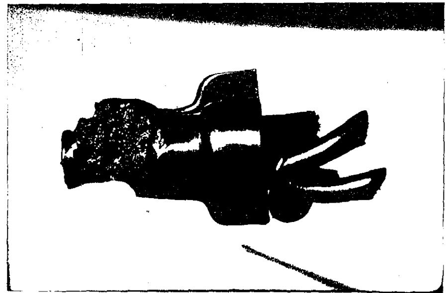
12. THIS FIELD FAILURE SHORTED TO GROUND when the thermoplastic insulating shell softened due to overheating in the connector spring area. Short circuits, due to insulation deterioration on the connector or wire, add to the fire hazard posed by the failure of aluminum-wired twist-on connections.
