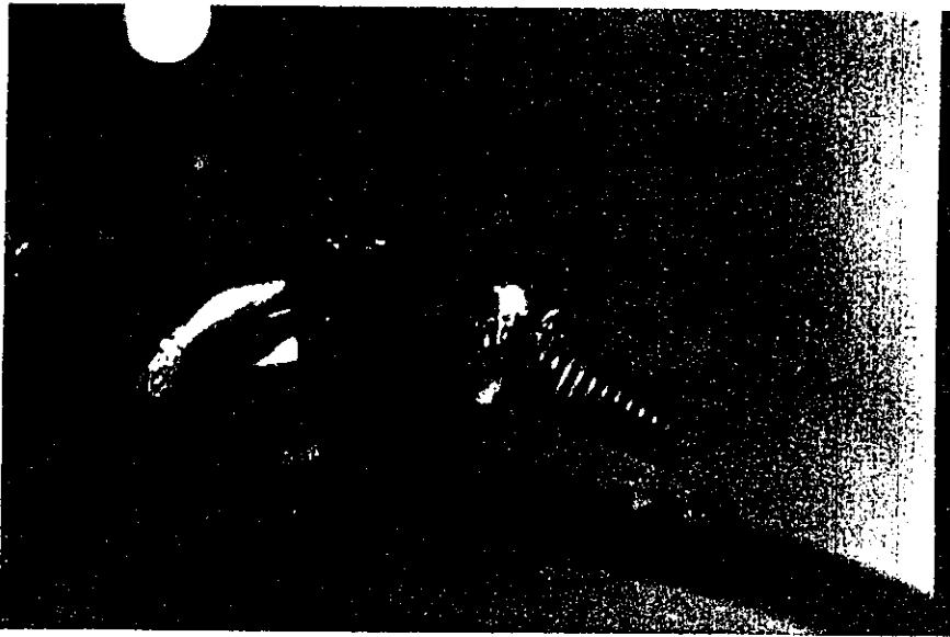
5. THE FIRE HAZARD POSED BY THESE SPLICES WHEN THEY FAIL IS EASILY SEEN WHEN THE "BURNOUTS" ARE OBSERVED WHILE PASSING CURRENT. At about 17 Amps, less than the 20 Amp rating of the (#10 aluminum wire) circuit, the connector spring is red hot. The voltage drop is about 2 volts, so downstream loads operate normally.
