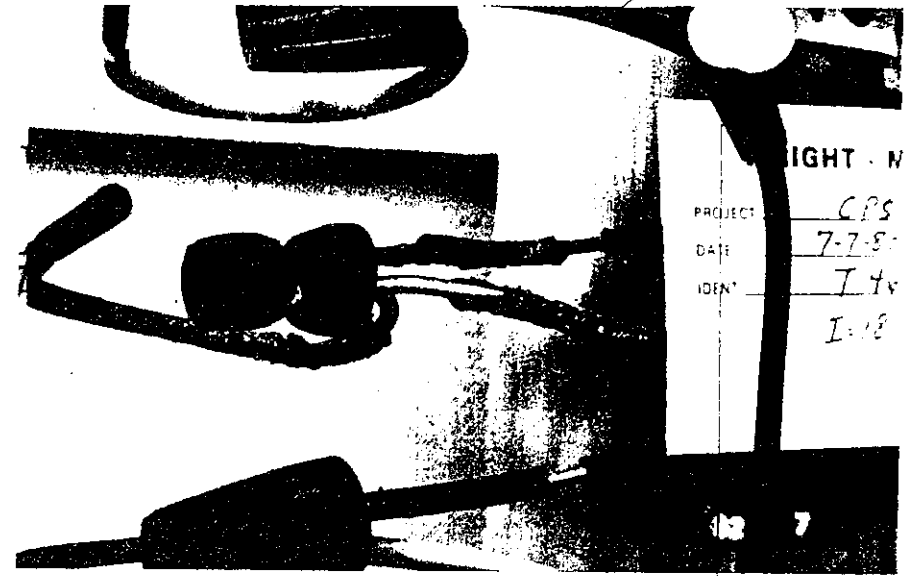
6. ADDITIONAL RED-HOT TWIST-ON CONNECTOR SPLICES FROM THE CPSC TESTS are shown here. The key point is that a significant percentage of the CPSC test splices, over a period of several years, failed in this hazardous manner, the spring becoming red hot. The connector shells ignited (smoldering combustion).
