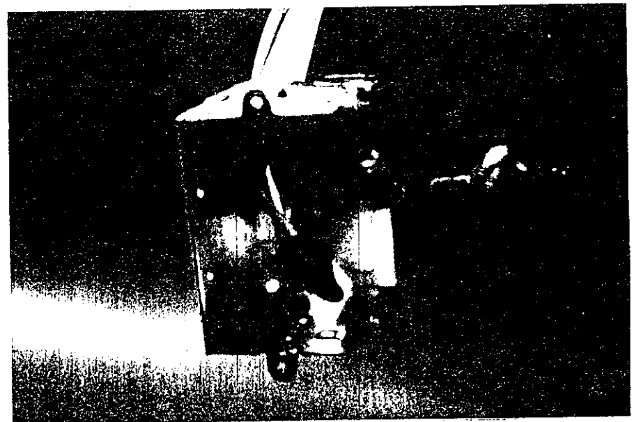
51. THE ONLY MATERIALS HERE ARE THOSE INTENDED TO BE IN THE BOX: the wires, a connector, and the end of the cable sheath. A failing aluminum twist-on splice can ignite its own shell. In this demonstration the connector shell was ignited by a match. A burning glob of plastic drips to the floor of the metal box.
