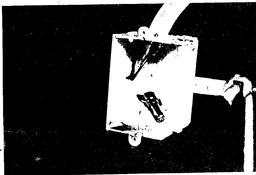
50. INSTALLED PER THE MANUFACTURER'S INSTRUCTIONS, MANY IN RETROFIT APPLICATIONS, hazardous failures will occur in considerable numbers over the years. The free-burning connector shell is then a cause for concern. A substantial fire can grow from ignition of a connector shell, as shown in this demonstration.
