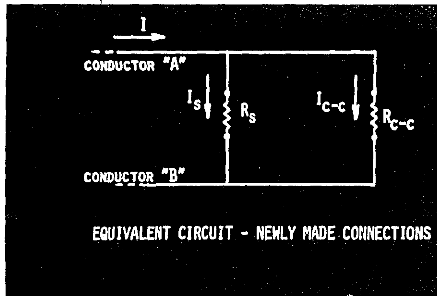
23. Combining the bulk resistances of the sections of the spring that are in parallel in the current path further simplifies the equivalent circuit for newly-made connections.
