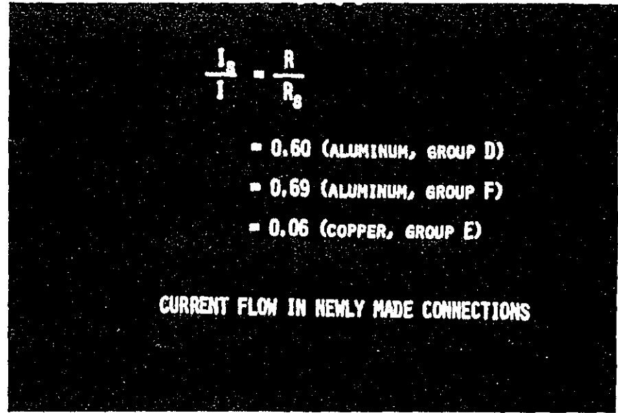
24. MEASUREMENTS ON NEWLY MADE ALUMINUM-WRED TWIST-ON SPLICES SHOW THAT MOST OF THE CURRENT FLOWS THROUGH SECTIONS OF THE STEEL SPRING. More than 60% typically for an aluminum connection but less than 10% in an all-copper connection. There is a basic difference in behavior with aluminum wire.
