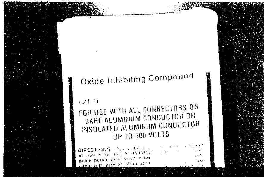
37. THE INHIBITOR USED SHOULD BE ONE THAT DOES NOT IGNITE AND FLAME READILY. Such compounds are commercially available. , shown here, is one of them.
