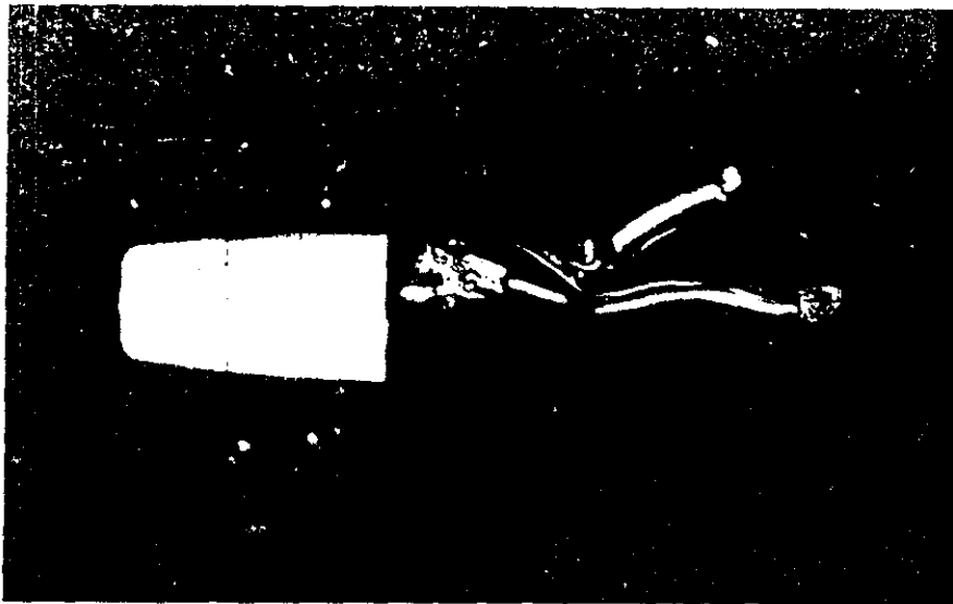
11. THE EARLIEST VISIBLE SIGN OF OVERHEATING is often softening and melting of the wire insulation, as in this field failure.
