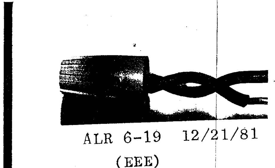
8. SIMPLER SPLICES ALSO FAILED. Here is a basic splice with two aluminum wires. Overheating is evident in the discoloration band around the shell. This is a characteristic heating pattern for failing aluminum wire twist-on splices. With time, further degradation occurs, and fire hazard develops with current loading.
