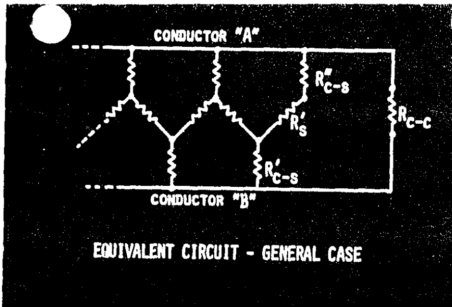
21. HERE IS THE MOST GENERAL EQUIVALENT CIRCUIT FOR THE TWIST-ON CONNECTOR
