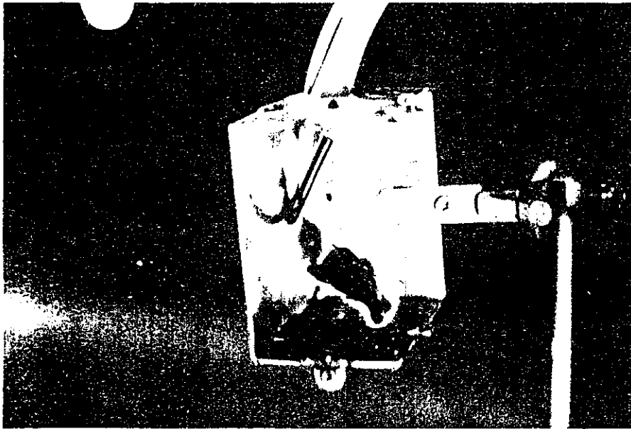
52. THE FLAME DOES NOT EXTINGUISH. Interaction between the shell and the dripped plastic keeps it going. In an actual installation the side and front of the box would be enclosed, but there are generally enough openings and gaps to provide sufficient air for combustion.
