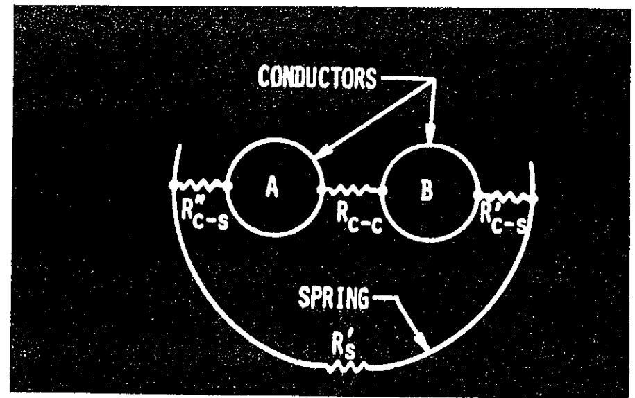
20. HERE ARE THE CURRENT PATHS IN THIS TYPE OF CONNECTION. Each of the paths from wire to wire has some associated resistance. The direct wire to wire path has only contact resistance, while paths through the spring sections have contact resistance as well as bulk resistance of the steel spring wire.
