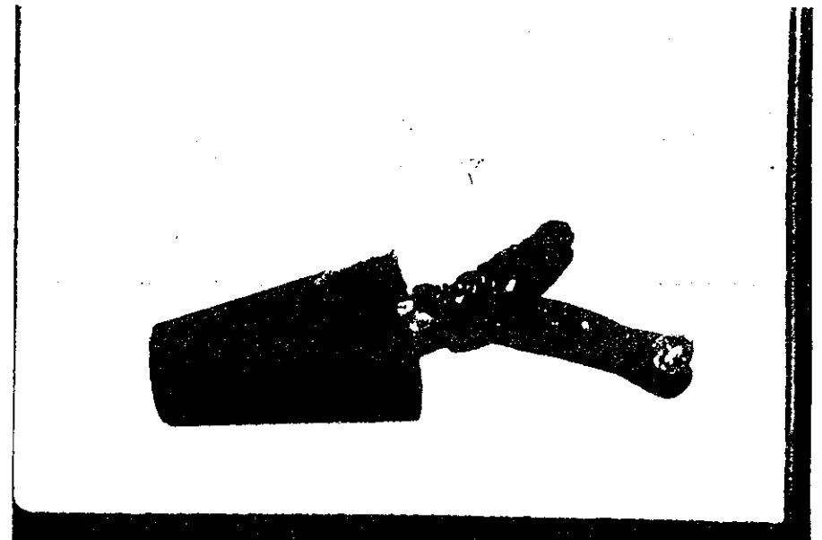
14. THIS FIELD FAILURE WAS IN SERVICE 9 YEARS. Failure of the aluminum-wired twist-on splices occurs in a relatively short time for a component of the permanent built-in wiring system of a home.
