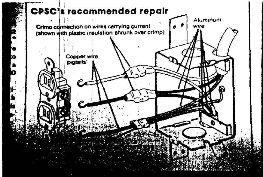
34. HERE IS AN ILLUSTRATION OF THE PIGTAILING METHOD USING THE COPALUM CONNECTOR.
