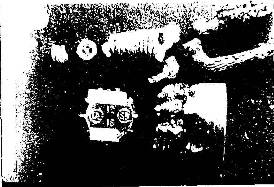
32. THIS SPECIAL SERVICE TWIST-ON SPLICE, BETWEEN ALUMINUM WIRE AND STRANDED COPPER WIRE, BURNED UP.
