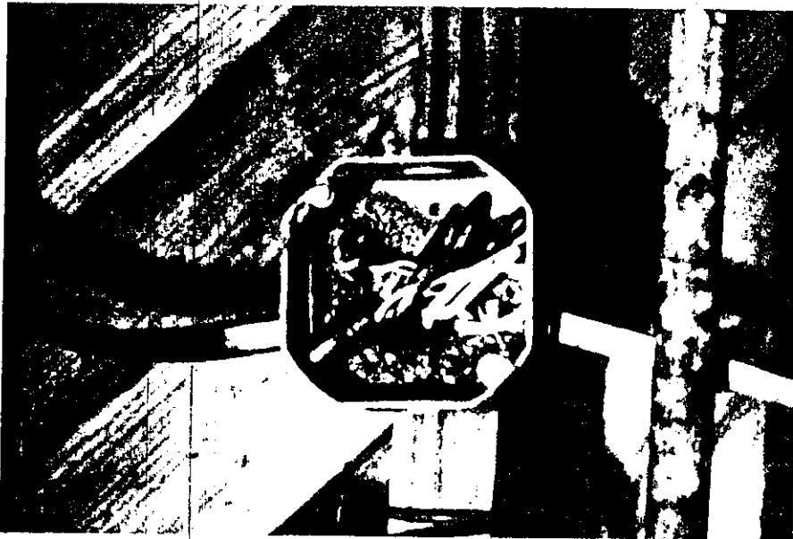
15. NOTE THE BURN-BACK OF THE WIRE INSULATION and the characteristic discoloration pattern on the connector shell of this field failure.
