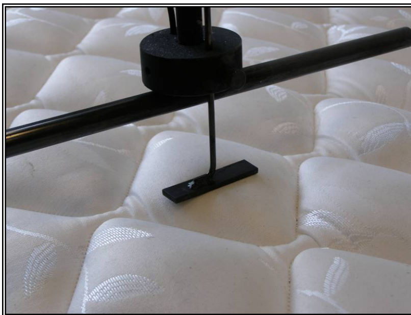
Figure 28. Step 25 Burner stand-off foot should not be in a depression.
