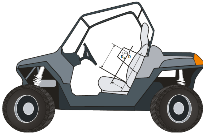
Figure 2. Point R in Shoulder/Hip Area 42
