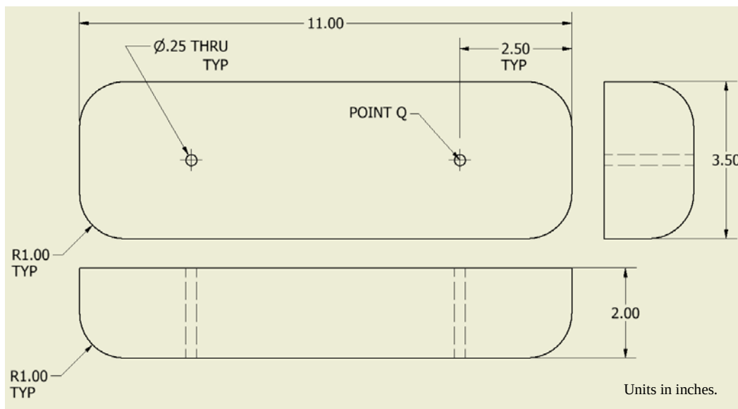
Figure 38: Shoulder/Hip Probe.
