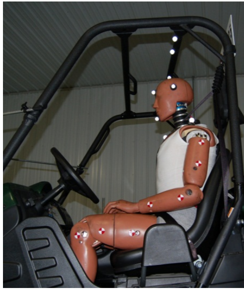
Figure 31: Vehicle H Side View
