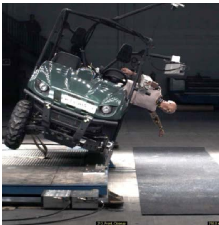
Figure 9: Deceleration Sled
