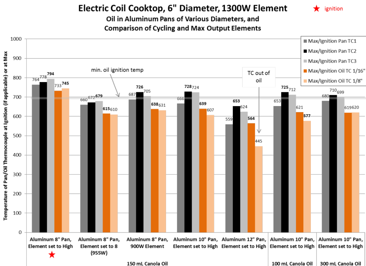
Figure 3: Results of Low Input Testing on Electric Coil Cooktop – Aluminum Pans
