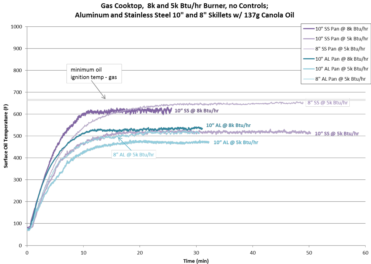
Figure 17: Oil Temperatures Reached From 5,000 and 8,000 Btu/hr Gas Burners
