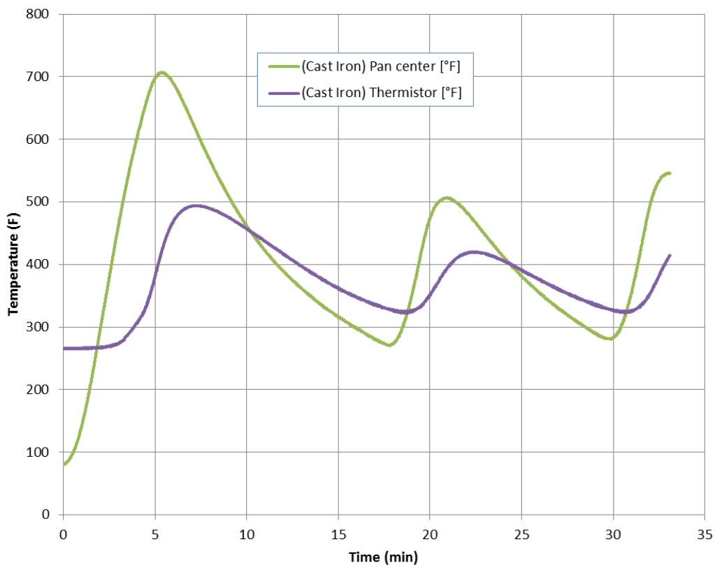
Figure 30: Dry-Cook Control of a 10” Cast Iron Pan on an Electric Coil Element using the High-Insulated Thermistor Sensor
