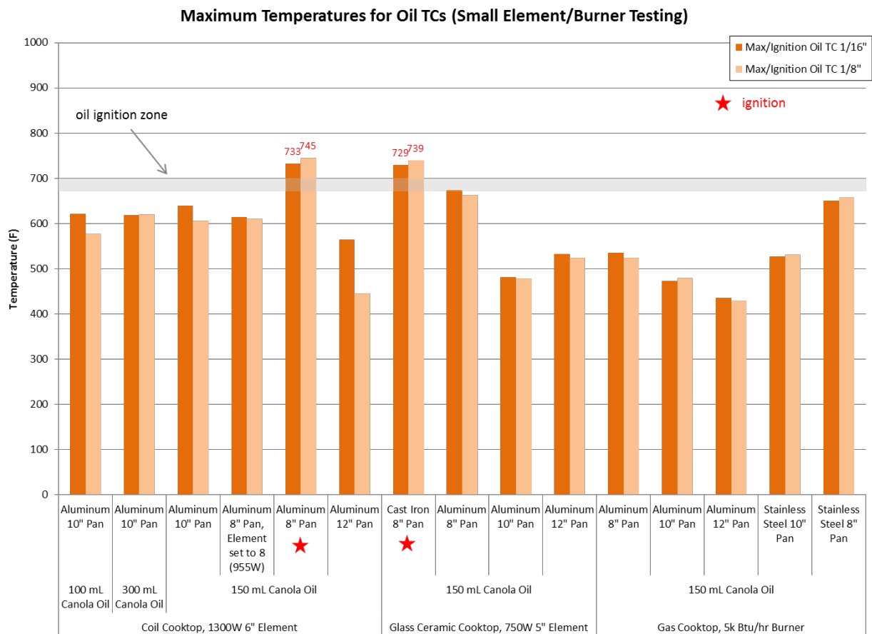
Figure 18: Summary Oil Temperature Results for 8", 10" and 12" Pans on All Cooktops
