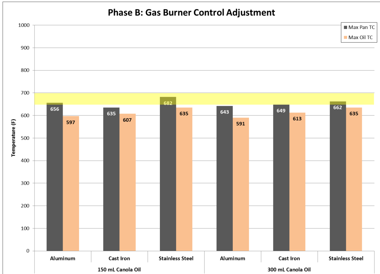
Figure 21: Maximum Pan and Oil Temperatures Reached on Gas Cooktop using 4,400 Btu/hr for Control (Reduced) Input Rate
