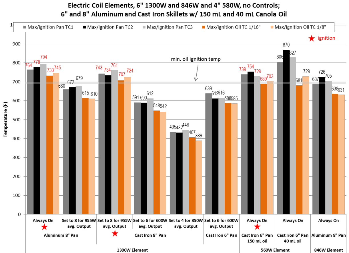
Figure 12: Summary of 8" and 6" Pan Tests at Low Average Power
