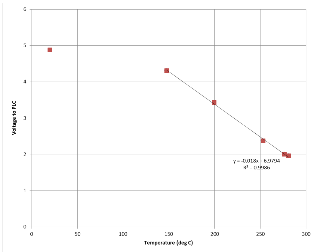
Figure 25: Typical Thermistor Calibration Curve, Showing Region of Linearization
