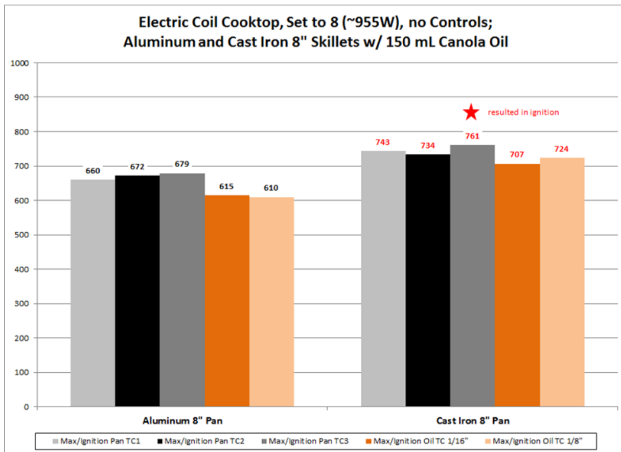
Figure 5: Comparison of Pan and Oil Temperatures, Cast Iron vs. Aluminum, No Controls
