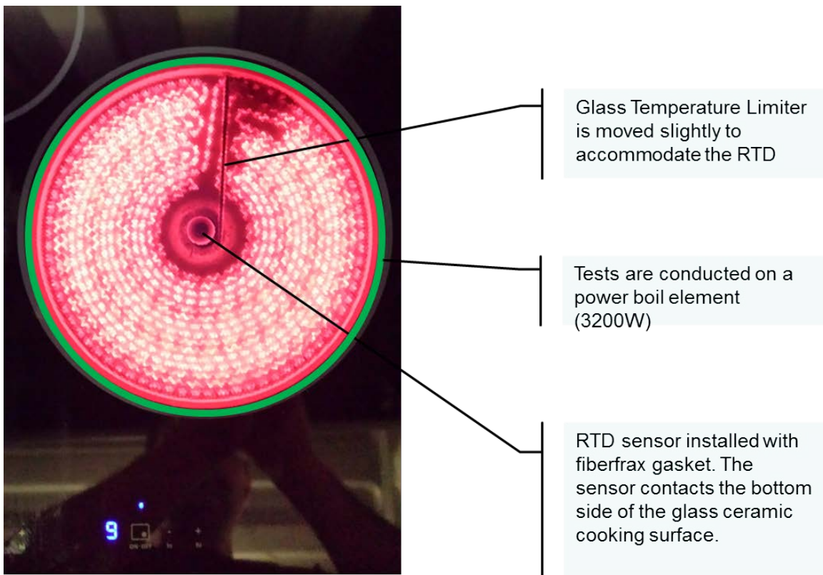
Figure 33: Sensor and Limiter Locations in 3200 W Element of Glass Ceramic Cooktop
