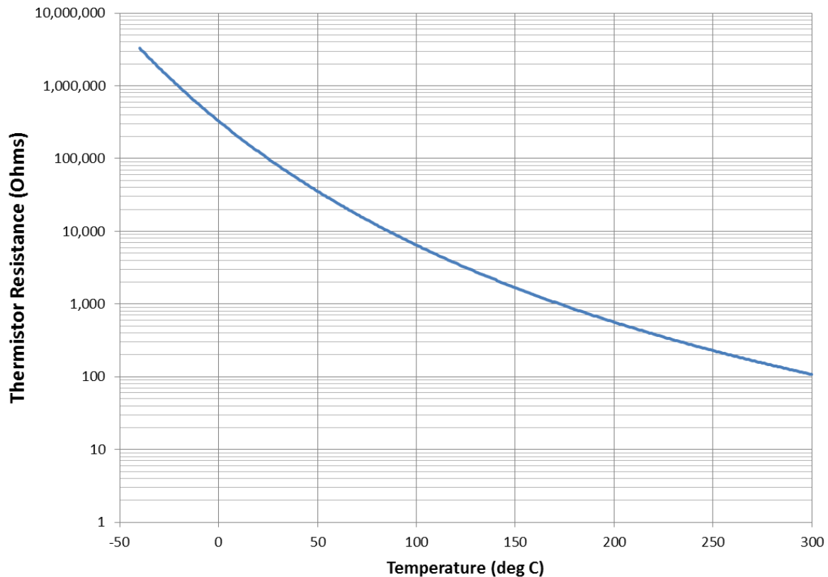
Figure 22: Representative Thermistor Resistance Curve
