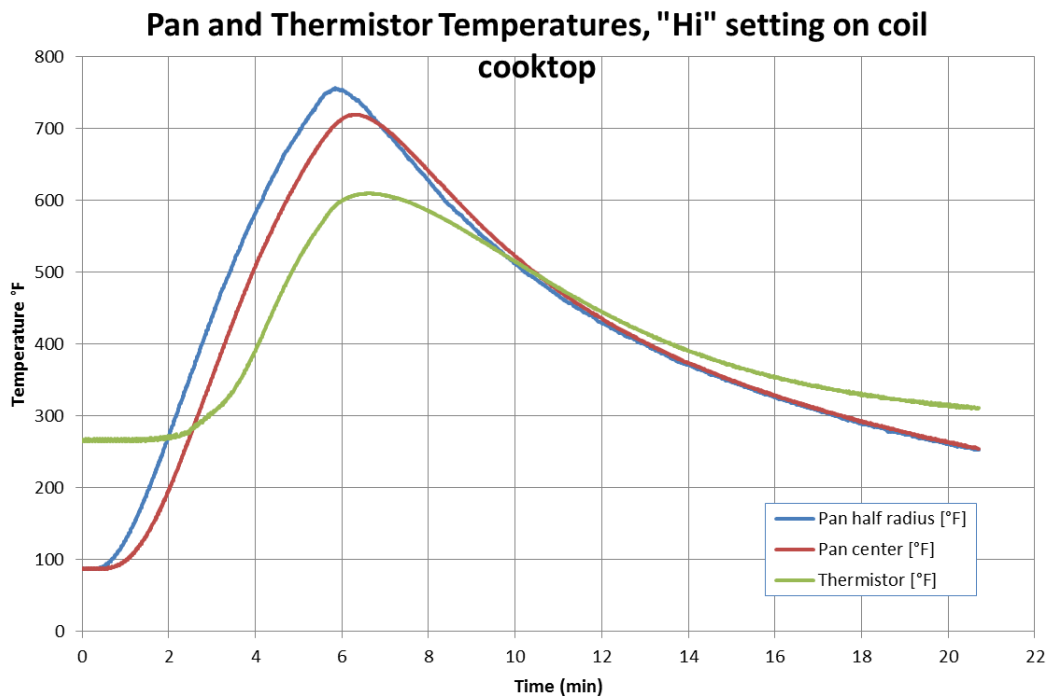
Figure 27: Pan and Thermistor Temperature Data for Dry Cook with 10" Cast Iron Pan on 8" Electric Coil on High. (Element shut off after approximately 5.5 minutes).
