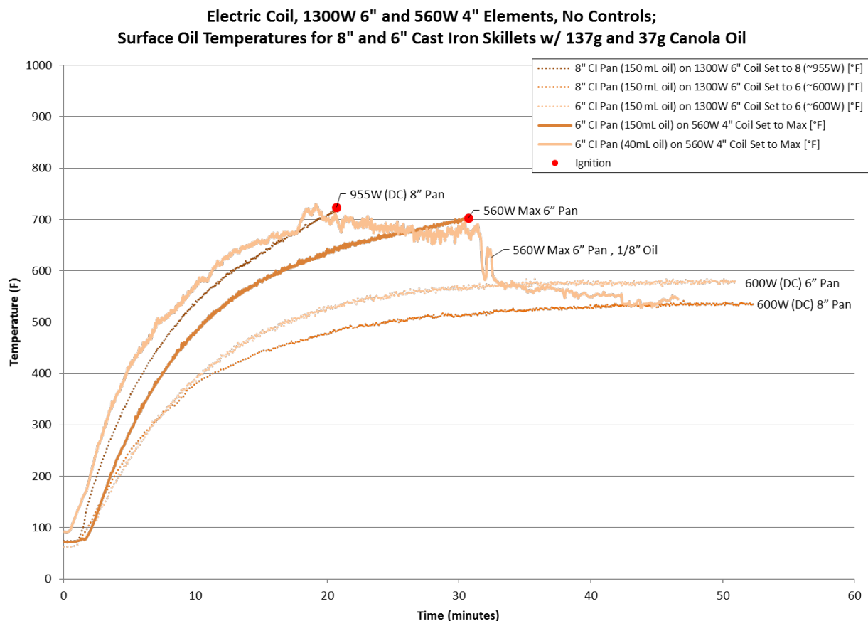
Figure 11: Oil Temperature Profiles for Duty Cycled vs Steady Power
