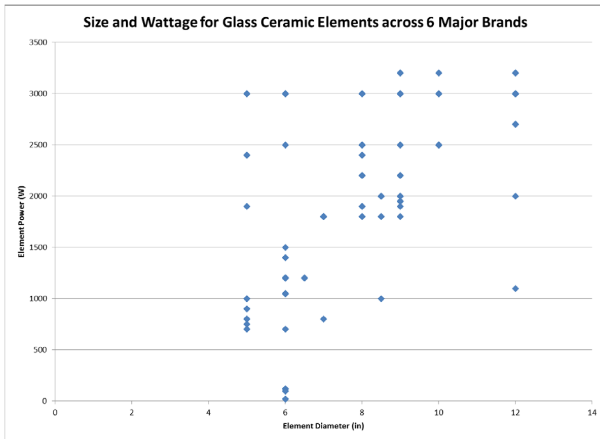
Figure 14: Scatter Plot of Glass Ceramic Cooktop Element Wattage and Diameter
