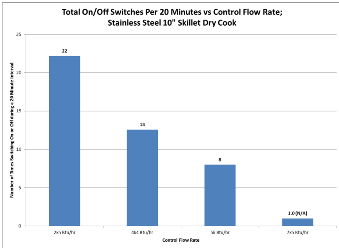
Figure 20: Relationship between Gas Flow at the Reduced Rate and Gas Valve Cycles
