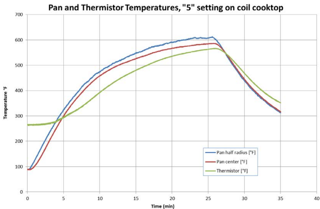
Figure 26: Pan and Thermistor Temperature Data for Dry Cook with 10" Cast Iron Pan on 8" Electric Coil at Setting 5. (Element shut off after approximately 27 minutes).
