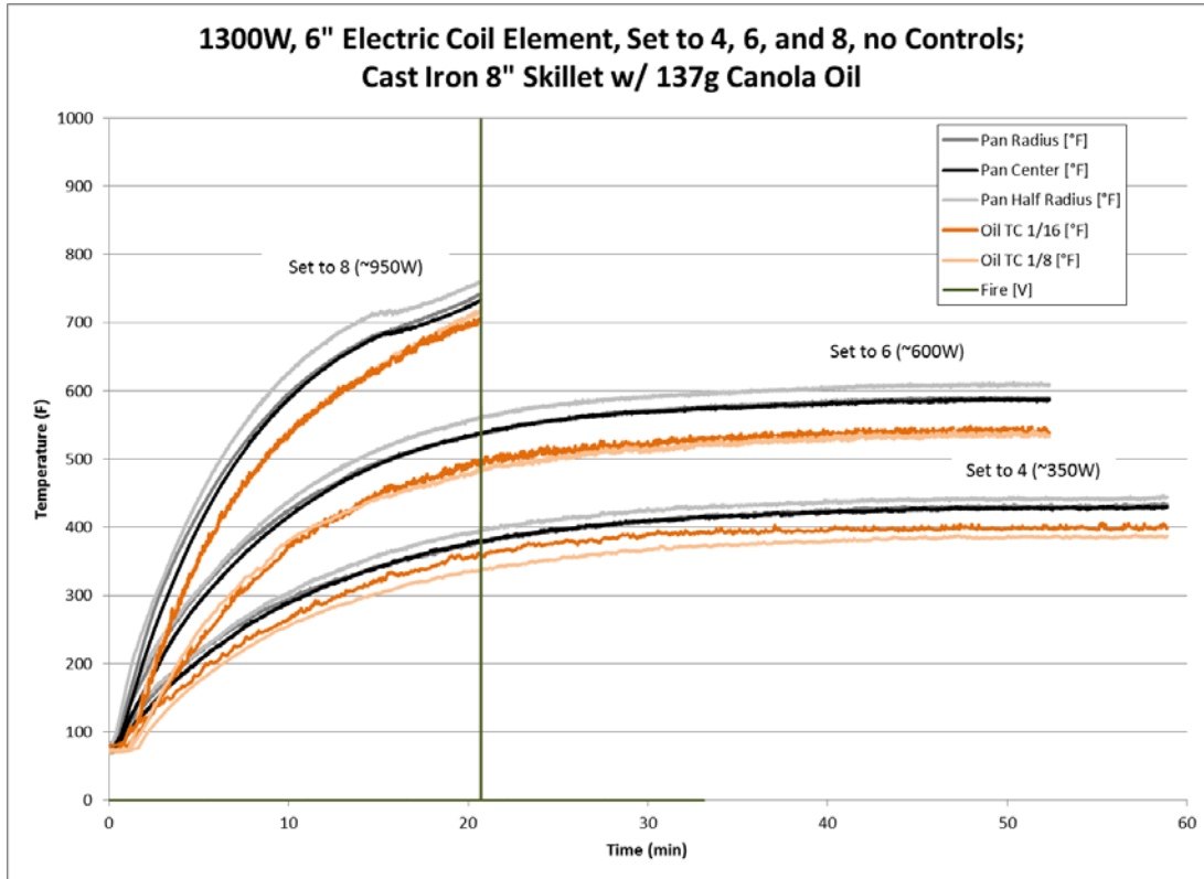
Figure 4: Electric Coil Element Set to “8”, “6” and “4” with a Cast Iron Pan
