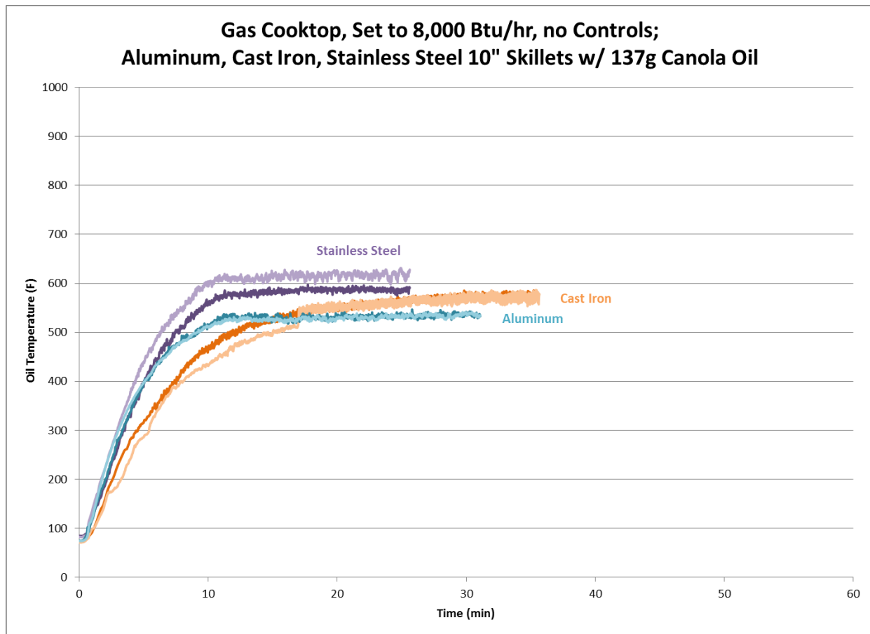
Figure 16: Oil Temperatures Reached From 8,000Btu/hr Burner on Gas Cooktop
