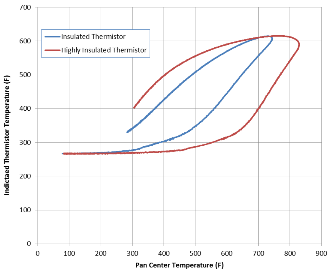
Figure 29: Impact of Additional Insulation on Response Characteristics of Thermistor Sensor
