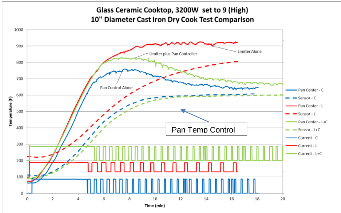
Figure 36: Dry Cook: Limiter Alone, Control Sensor Alone, Limiter plus Control
