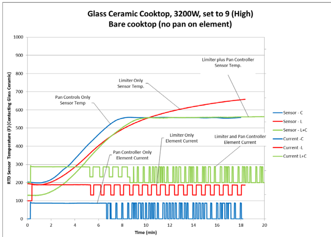
Figure 34: Bare Cooktop: Limiter Alone, Control Sensor Alone, Limiter plus Control
