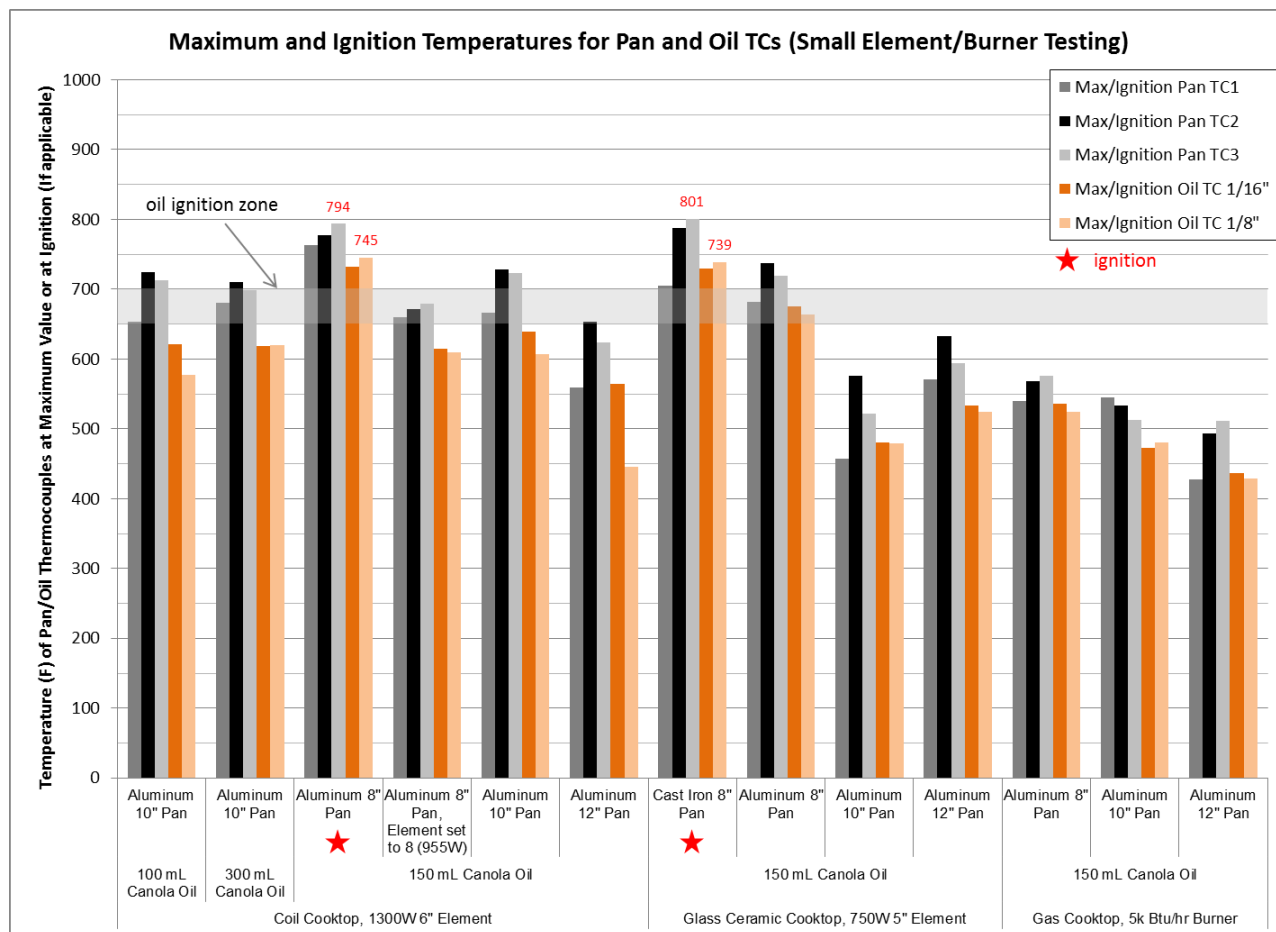
Figure 2: Results of Low Input Rate Testing – Initial Test Matrix
