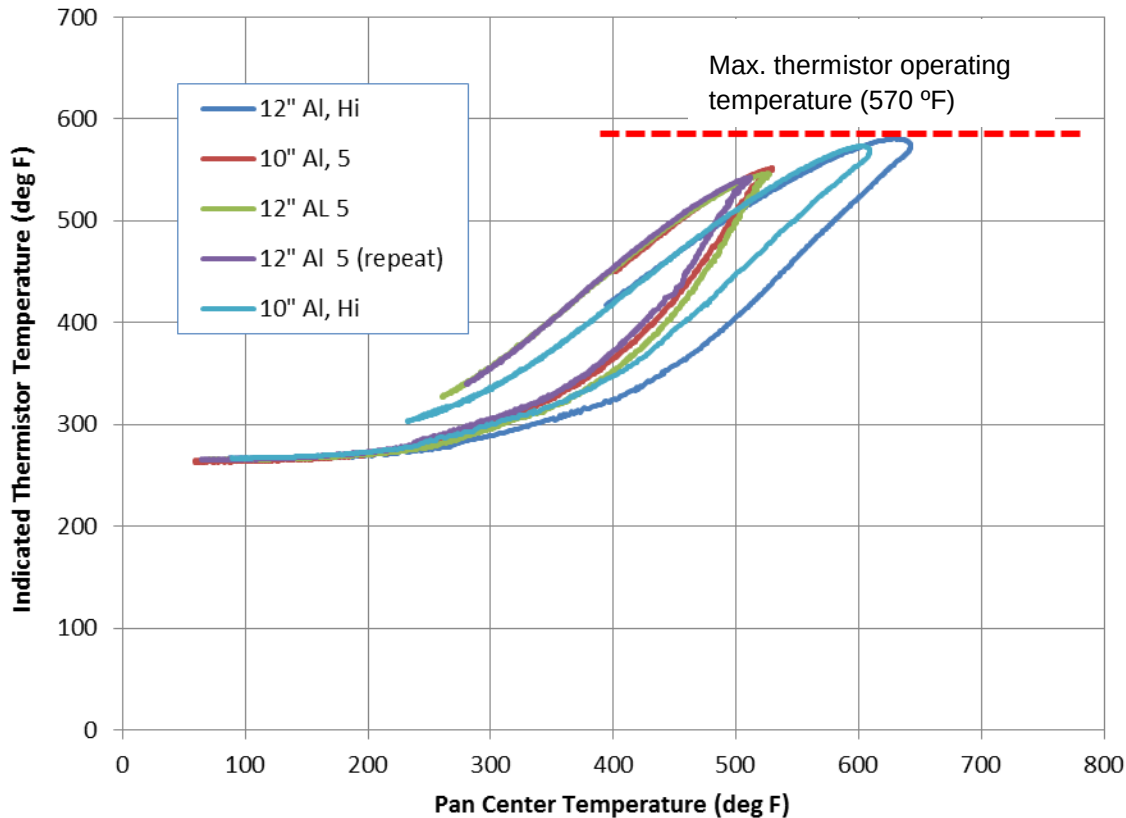
Figure 28: Indicated Thermistor Temperature as a Function of Pan Center Temperature for Various Pan Types and Heating Rates
