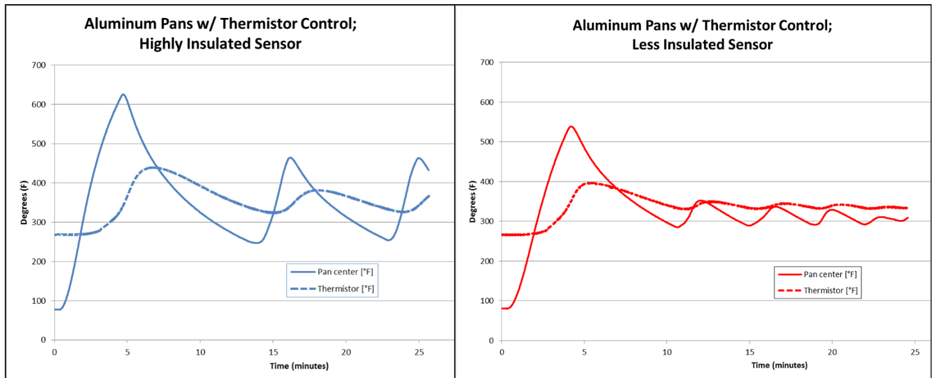
Figure 32: Pan Center Temperatures and Thermistor Temperatures for Two Different Sensor Body Arrangements
