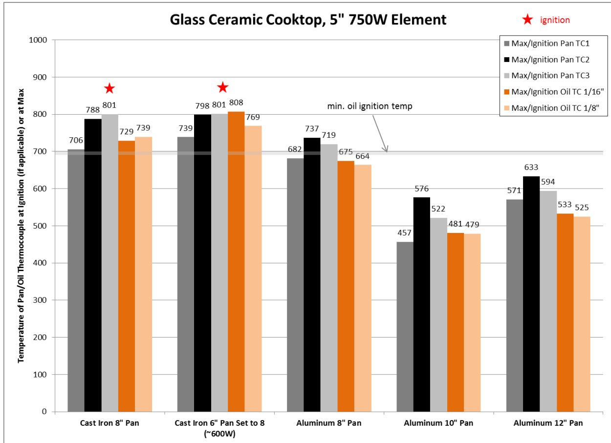
Figure 13: Results of Low Input Testing on Glass Ceramic Cooktop
