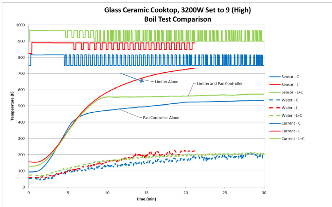
Figure 35: Water Boil: Limiter Alone, Control Sensor Alone, Limiter plus Control
