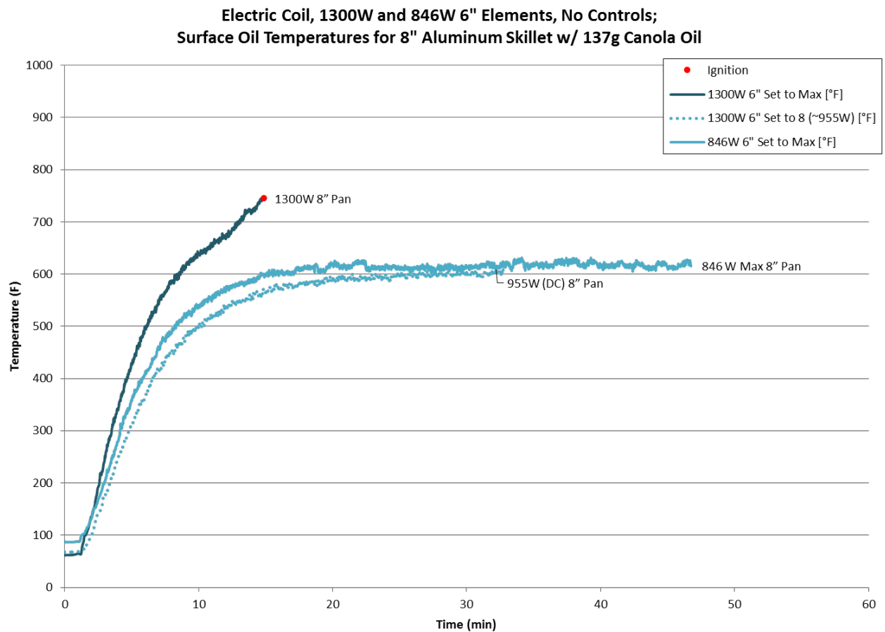
Figure 9: Oil Temperature Profiles in Aluminum Pans: Cycled Elements vs Full Powered Elements of Similar Wattage
