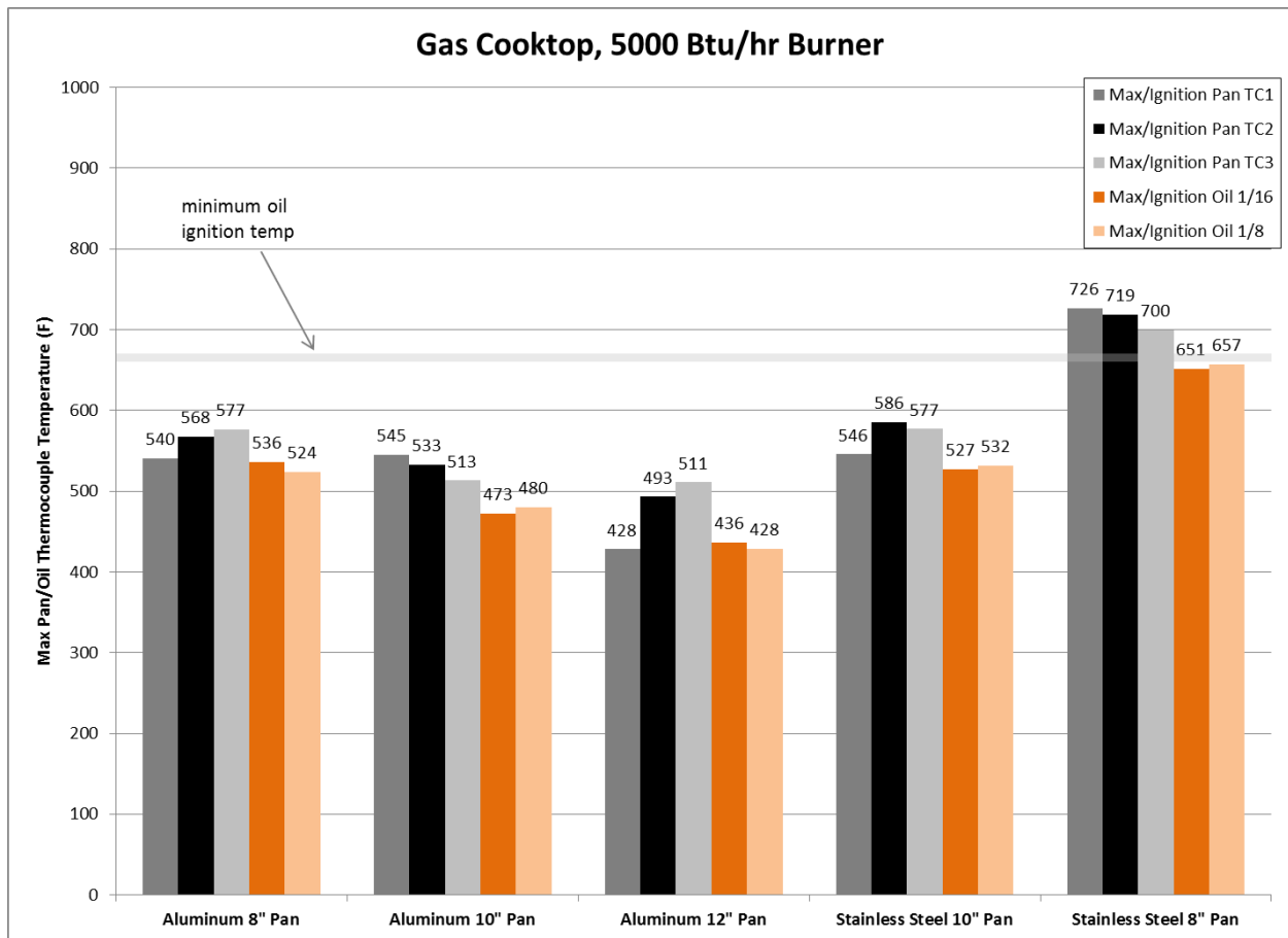
Figure 15: Results of Low Input Rate Testing on Gas Cooktop
