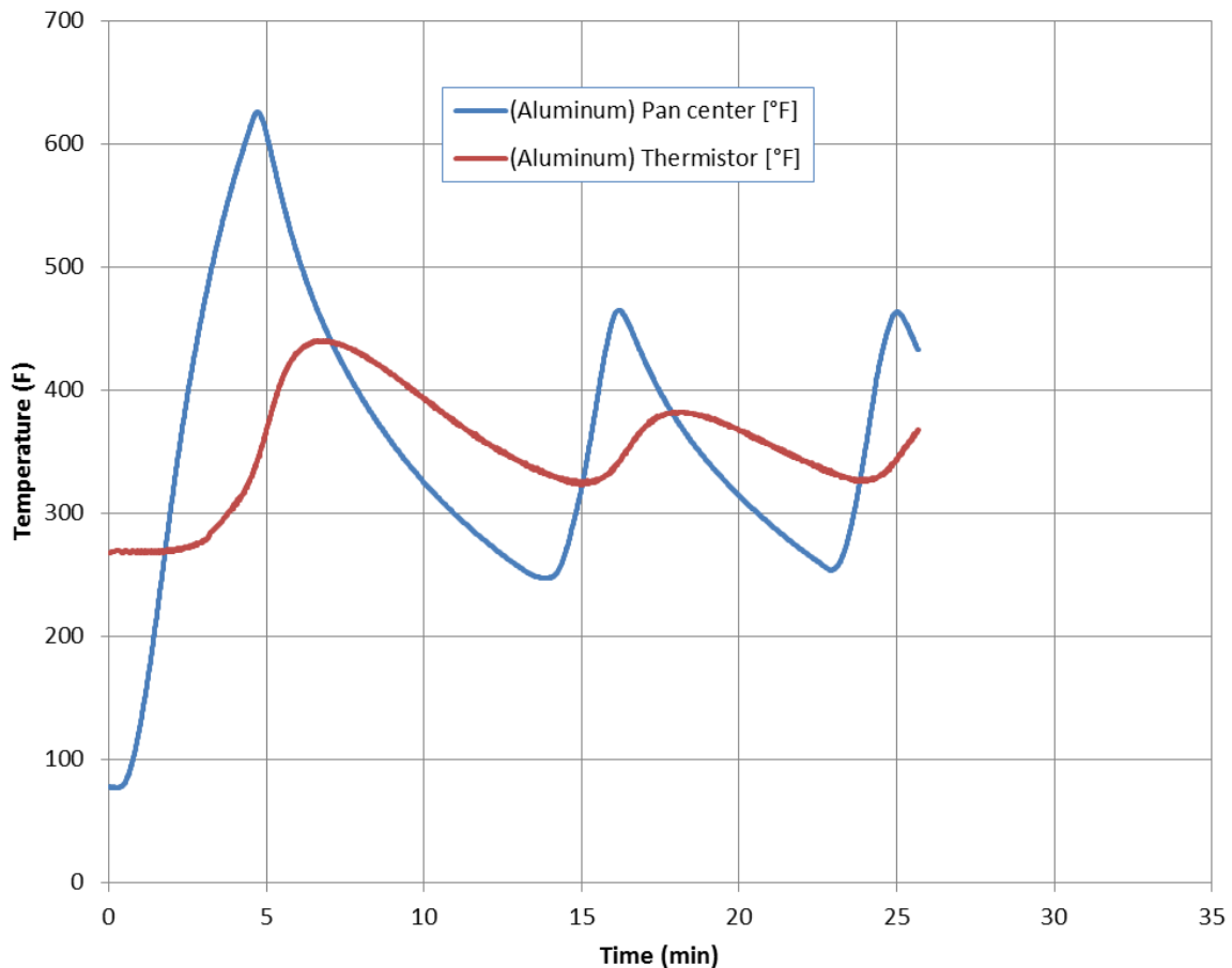
Figure 31: Dry-Cook Control of a 10" Aluminum Pan on an Electric Coil Element with the Highly-Insulated Thermistor Sensor
