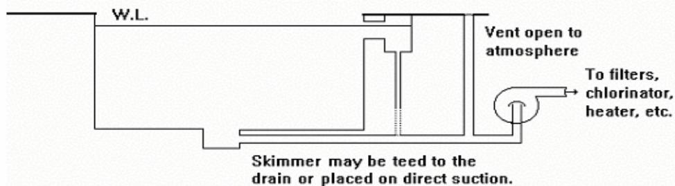
Figure 4. Vent System to relieve Main Drain Suction
