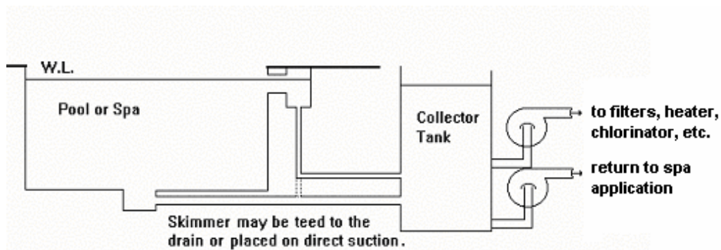
Figure 3. Gravity feed system - Direct Suction removed from Main Drain.
