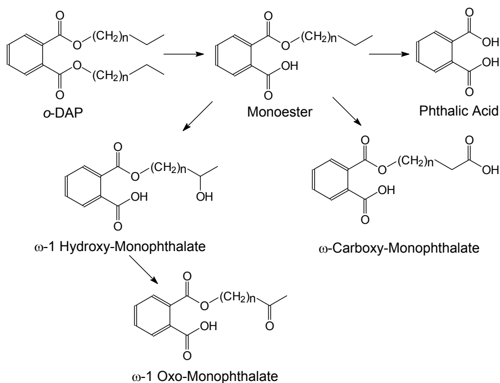
Figure 2. Metabolism of ortho -Dialkyl Phthalates ( o -DAP's). Adapted from Frederiksen et al. 2007.
