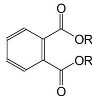
Figure 1. Dialkyl o -Phthalate
