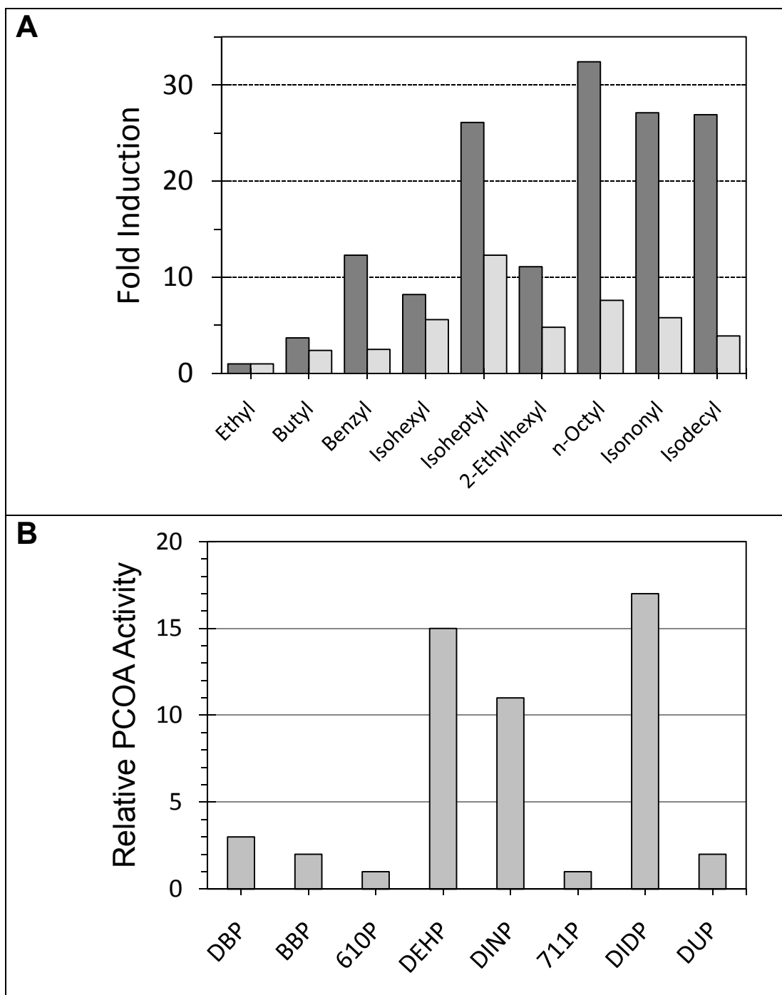
Figure 4. Induction of PPAR \alpha and peroxisome proliferation. A). In vitro activation of mouse (dark gray bars) or human (light gray bars) PPAR \alpha by the corresponding monoesters of the o -DAP's (Bility et al. 2004). B). In vivo induction of peroxisome proliferation, as palmitoyl CoA oxidase (PCOA) activity, by o -DAP's in rats (Barber et al. 1987). Note that the horizontal axes list different o -DAP's. 610P, mixture containing C6-C10 di- n -alkyl phthalates; 711P, mixture containing C7-C11 di- n -alkyl phthalates; DUP, di- n -undecyl phthalate.
