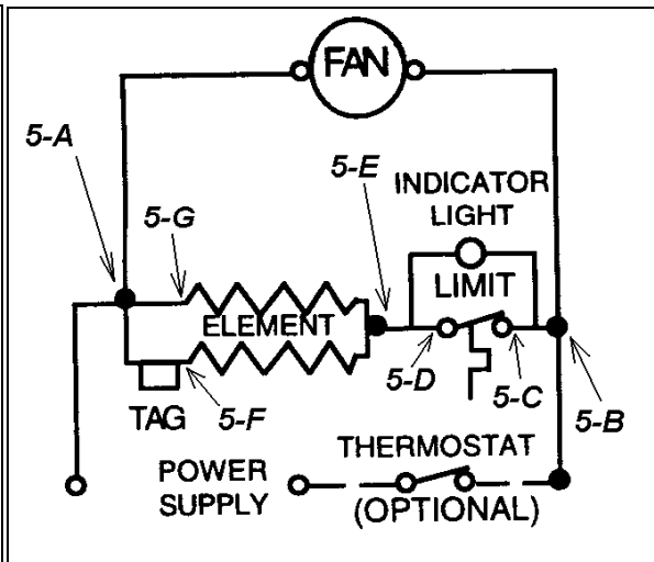
WIRING DIAGRAM*, HEATER #5
