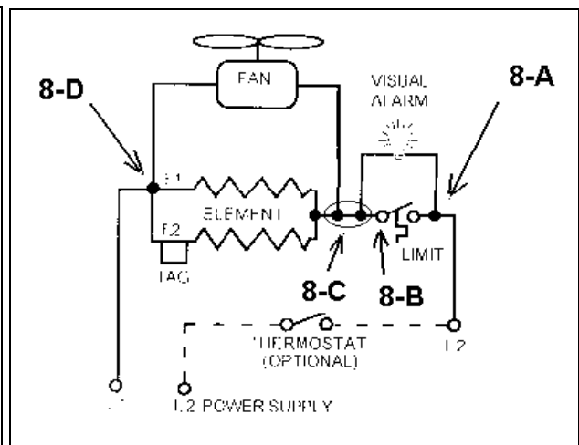
WIRING DIAGRAM*, HEATER #8
