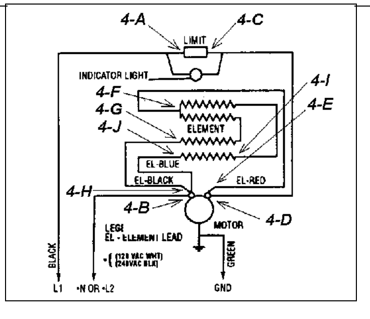
WIRING DIAGRAM*, HEATER #4
