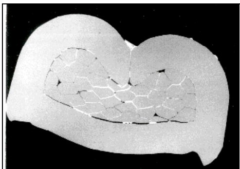
FIGURE 5-1 - CONNECTOR #4-D Resistance = 81 \mu\Omega
