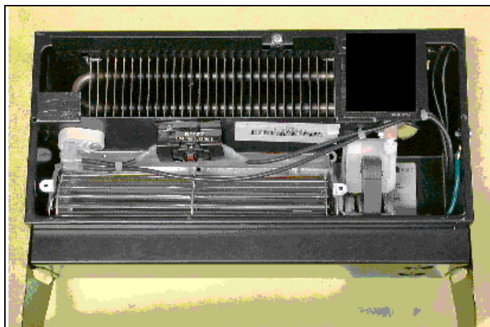
HEATER #9
