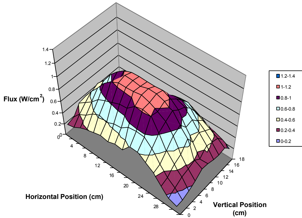
Figure 18: Heater C Flux Map, Sensor Position = 5 cm from the Heater Front
