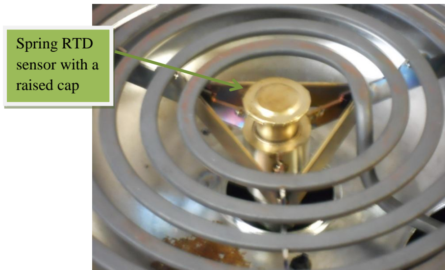
Figure 3: Spring Loaded RTD Sensor with Raised Cap
