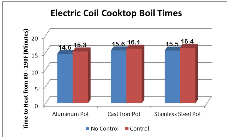
Figure 15: Water Heating Time Comparison, Electric Coil Cooktop
