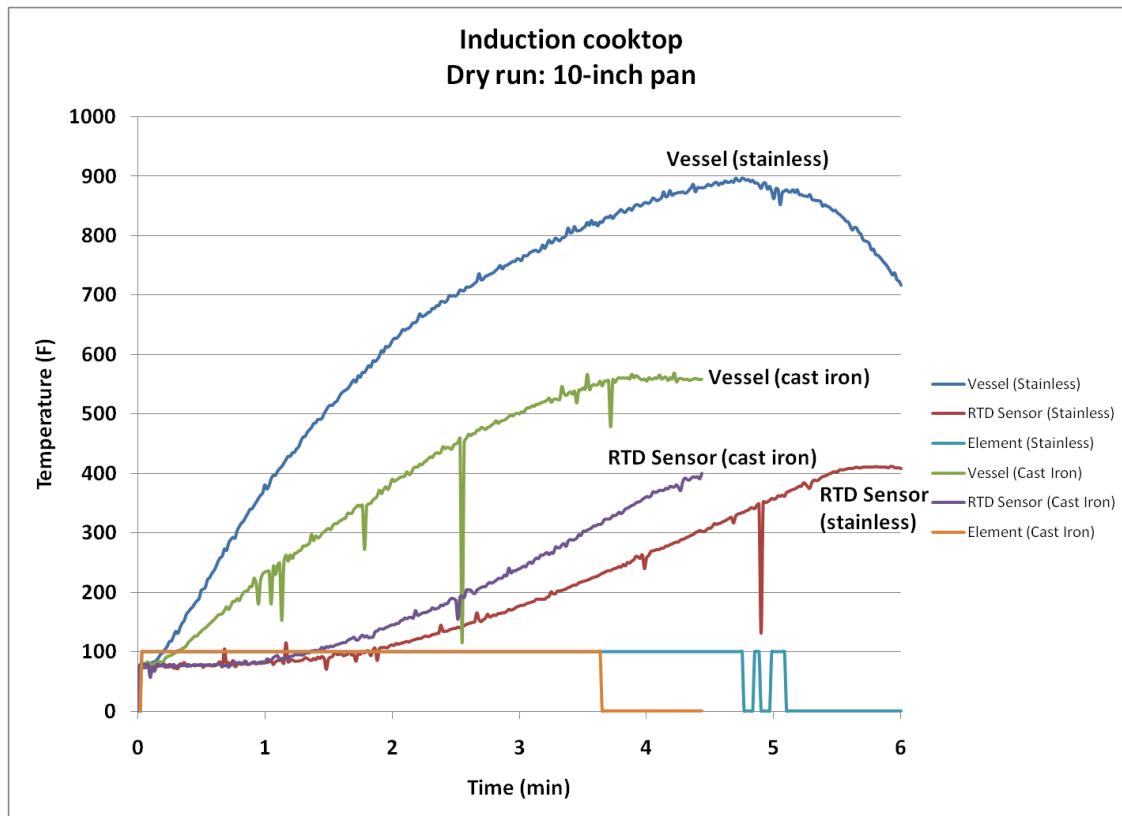
Figure 33: Existing Induction Cooktop Controls React to Pan Temperature
