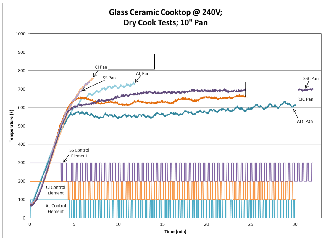
Figure 25: Glass Ceramic Cooktop – “Dry-Cook” Tests for Pan Temperature Limitation
