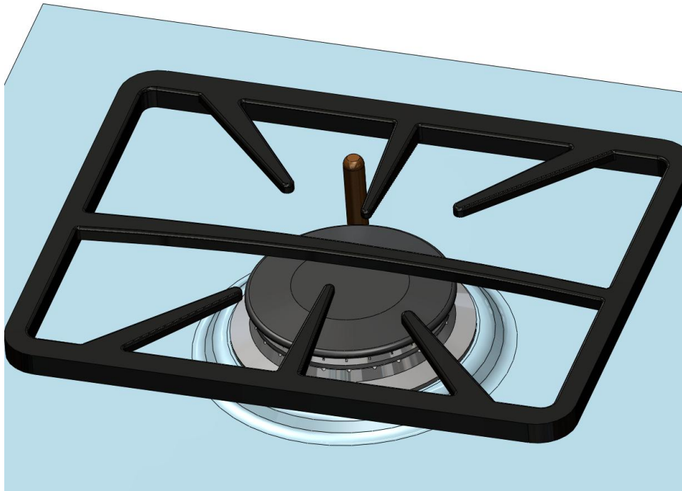
Figure 36: Schematic of Gas Cooktop with Embedded Sensor
