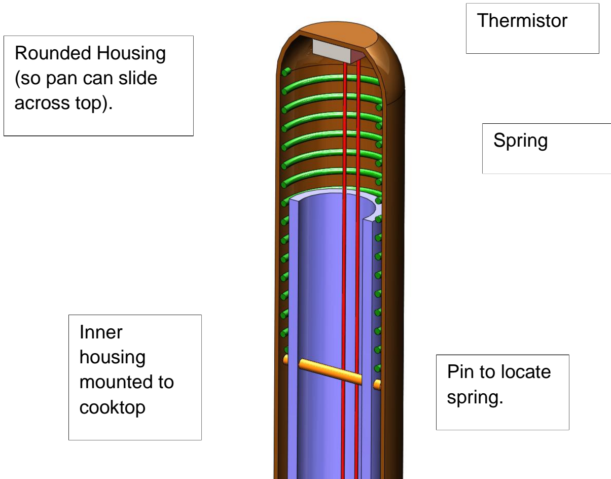
Figure 35: Details of Sensor Construction
