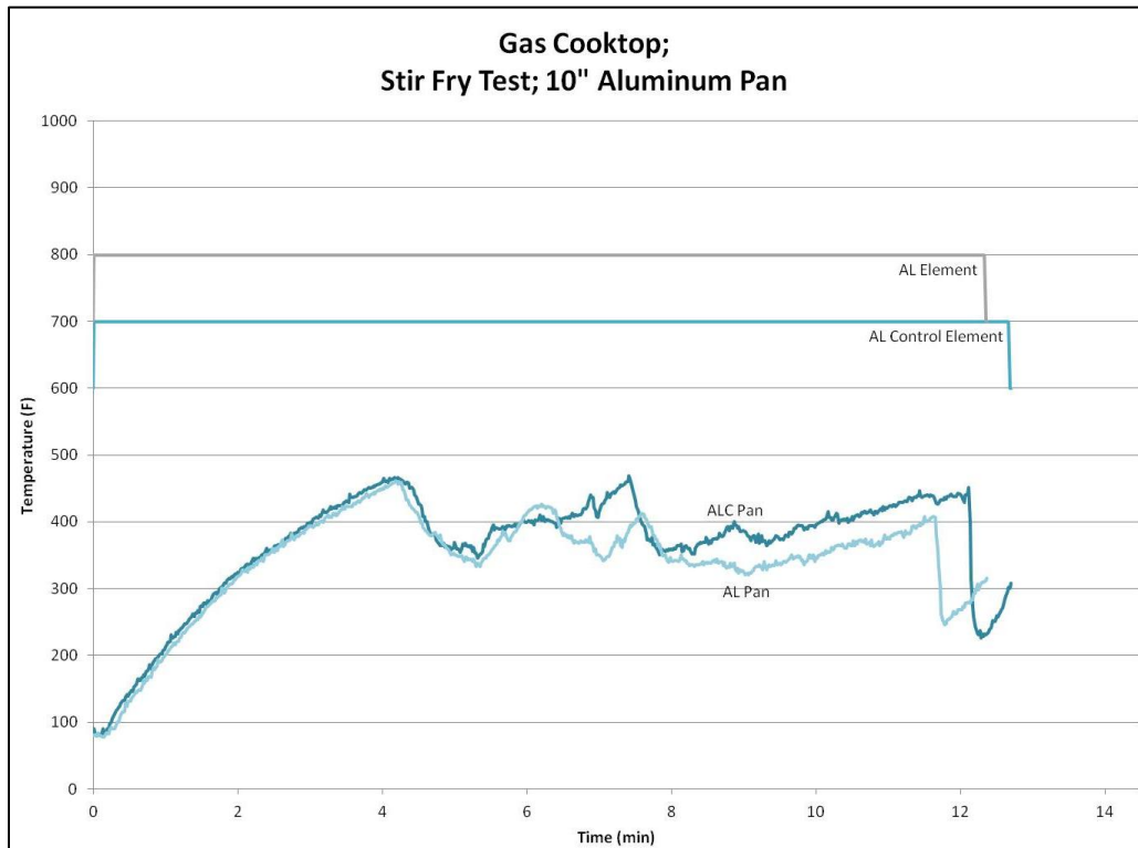
Figure 24: Gas Cooktop – Stir-Frying Vegetables in Aluminum Pan
