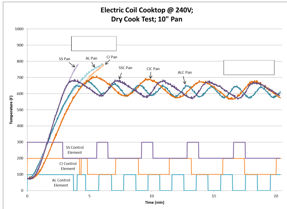
Figure 14: Dry Cook Results using the Electric Coil Cooktop
