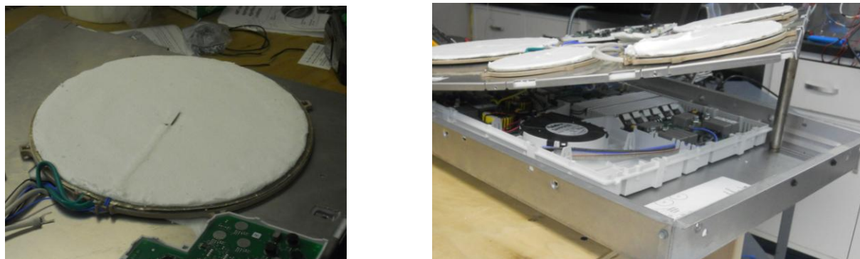
Figure 13: Induction Element with RTD, Induction Cooktop Electronics
