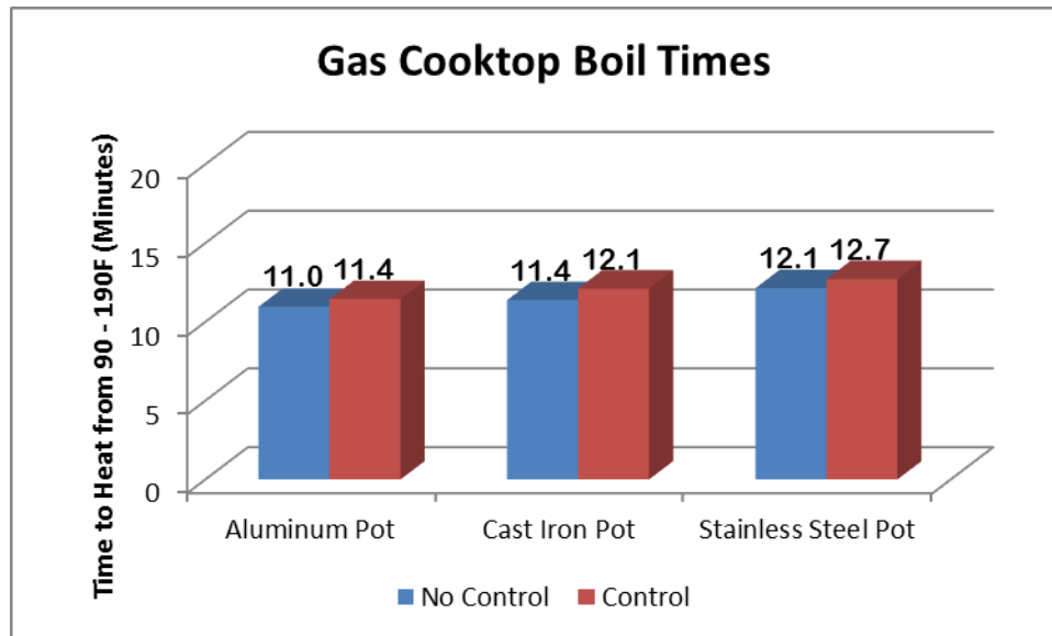
Figure 20: Gas Cooktop – Water Heating Time Comparison
