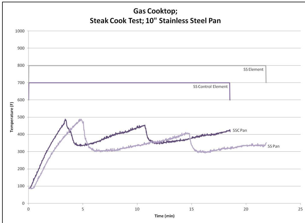
Figure 22: Gas Cooktop – Steak Searing with Stainless Steel Pan
