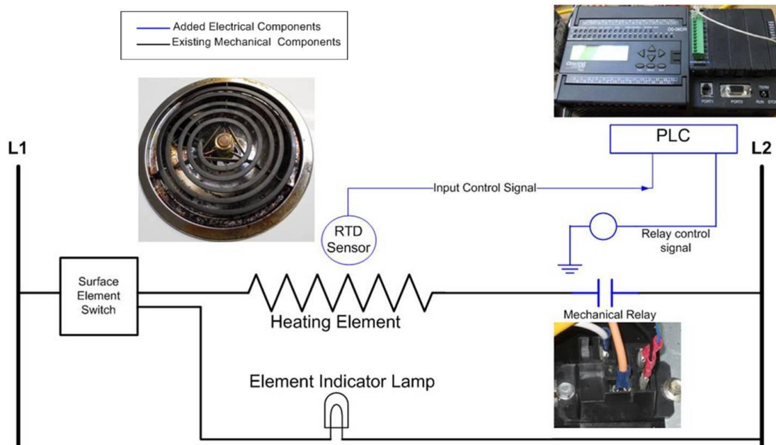
Figure 5: Electric Coil Cooktop Control System Hardware
