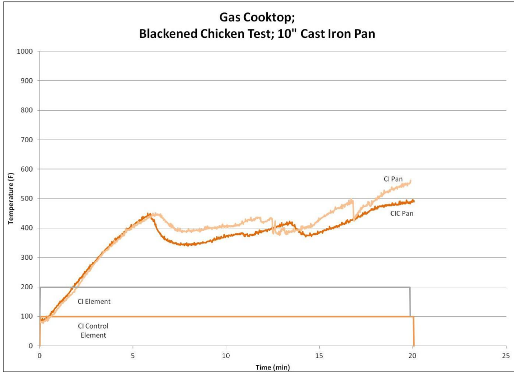
Figure 23: Gas Cooktop – Blackening Chicken in Cast Iron Pan
