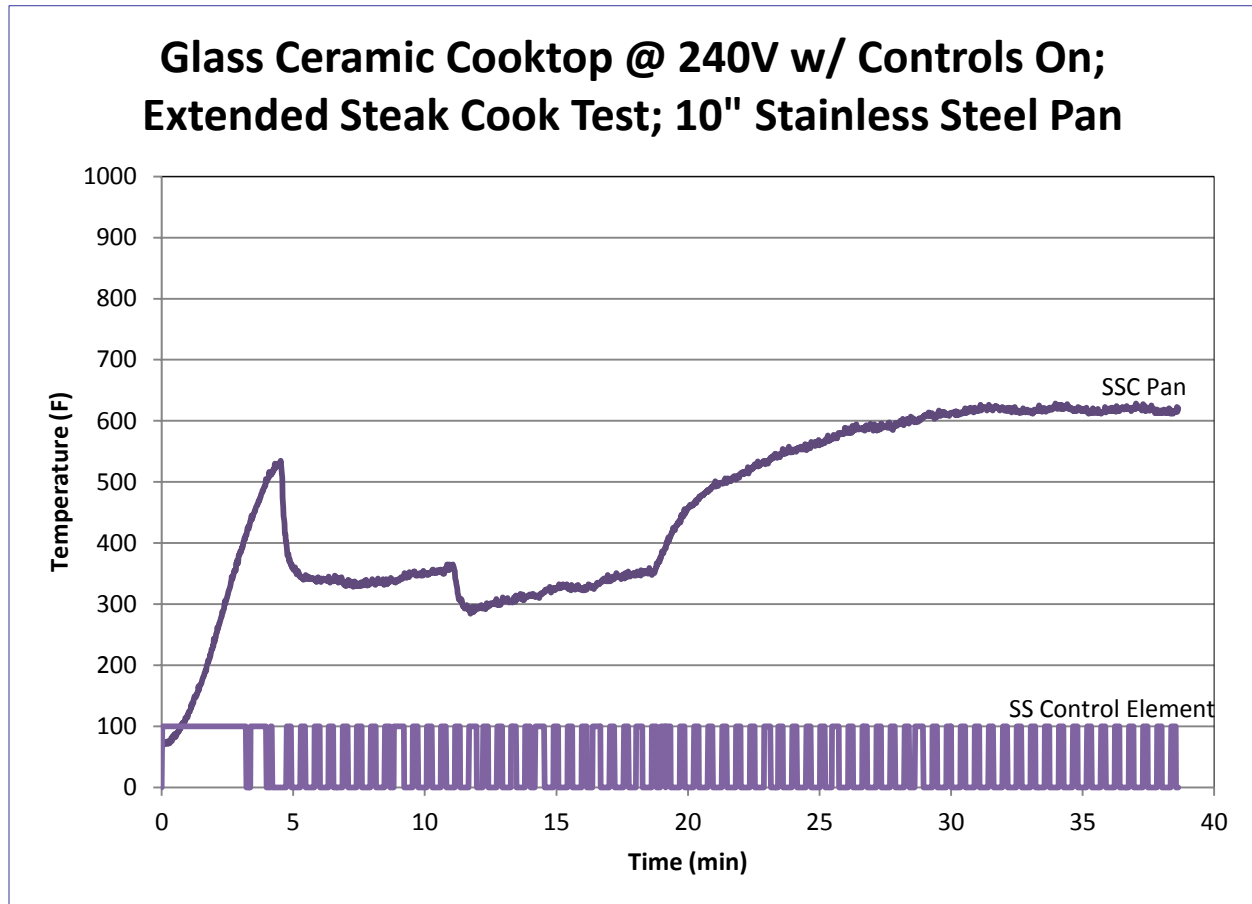
Figure 26: Temperature Limitation on Glass Ceramic Cooktop after Cooking Steak
