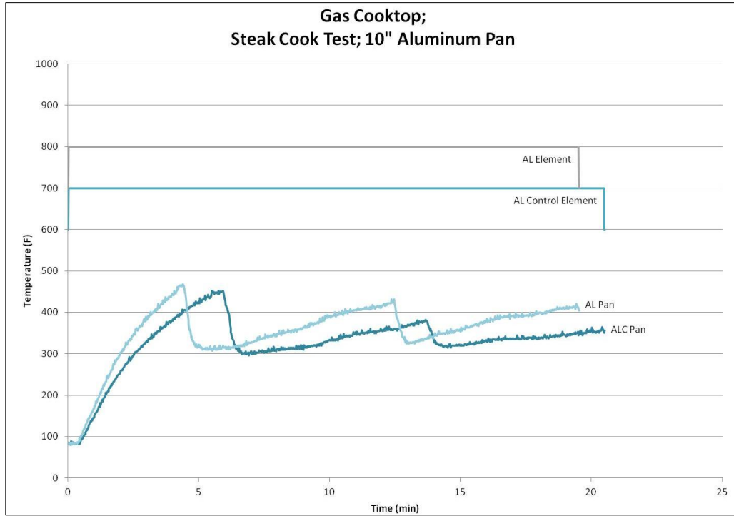
Figure 21: Gas Cooktop – Steak Searing with Aluminum Pan
