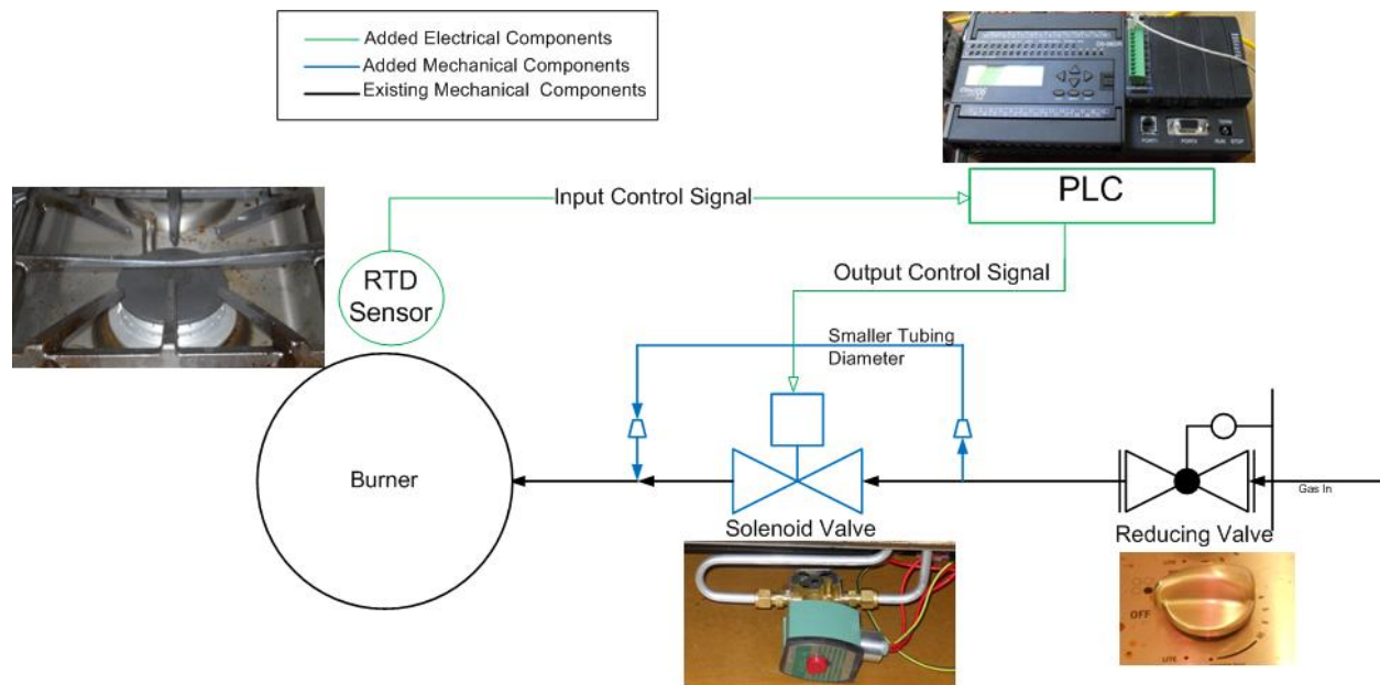
Figure 9: Gas Cooktop Control System Hardware
