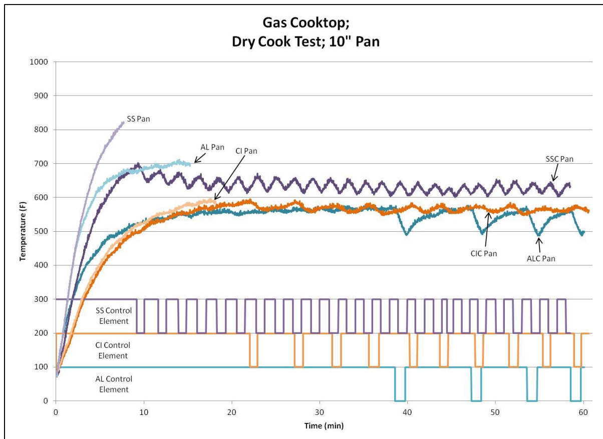
Figure 19: Dry Cook Results Using the Gas Cooktop with Controls Activated
