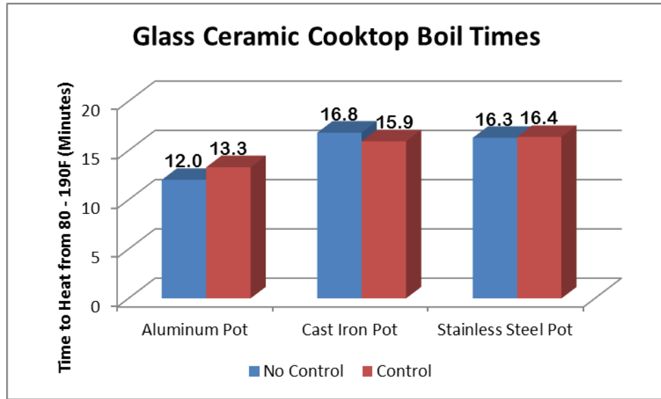
Figure 27: Glass Ceramic Cooktop – Water Heating Time Comparison,
