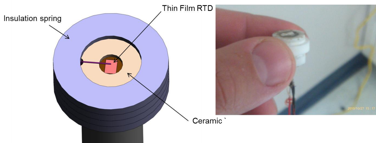
Figure 10: RTD Sensor Used Under Glass Ceramic Cooktop
