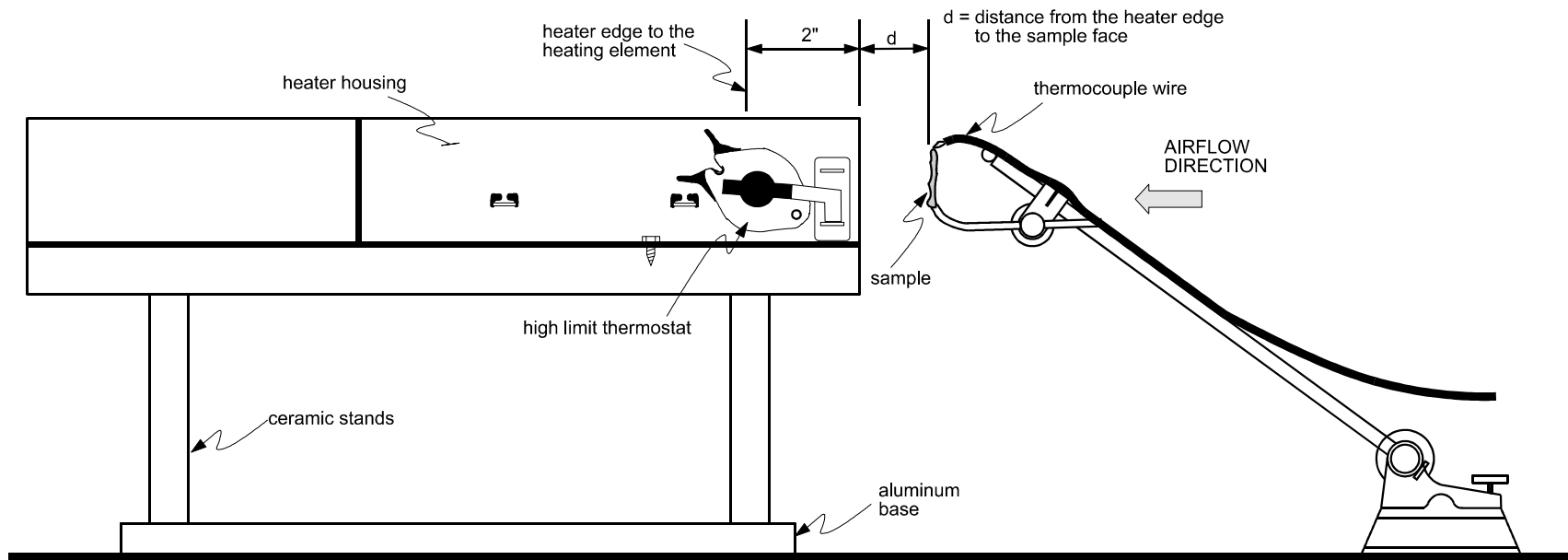
Figure G-1. Lint at Heater Intake Dimensions of the Test Setup
