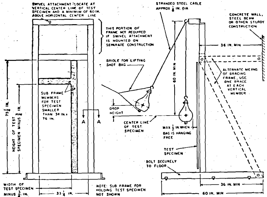
FIG 2-TEST FRAME
