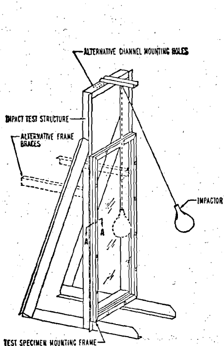
FIG 1-GLASS IMPACT TEST STRUCTURE
