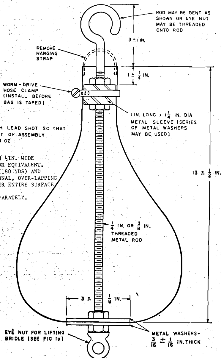
FIG 5 - IMPACTOR
