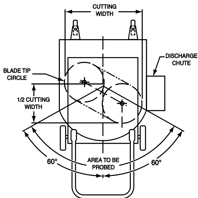
FIGURE 4 - AREA TO BE PROBED MULTI-BLADE MOWERS
