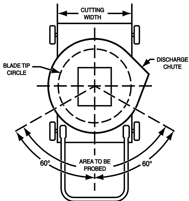
FIGURE 3 - AREA TO BE PROBED
