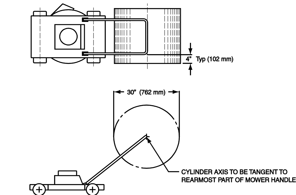
FIGURE 1 - OPERATING CONTROL ZONE
