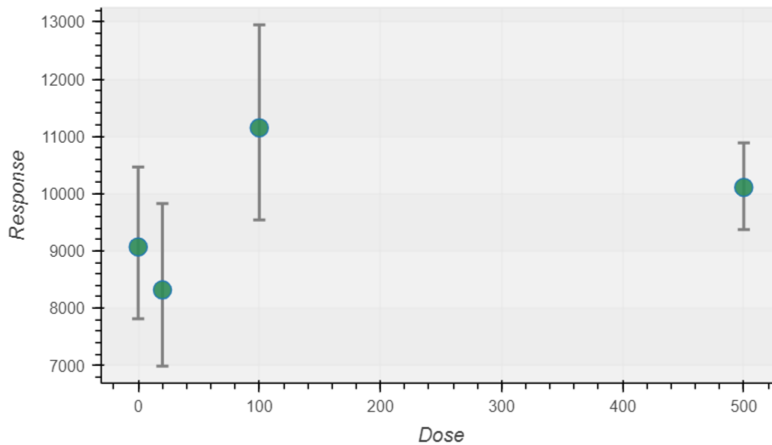
CO-9 Task 1B Attachment 2 - 28564613_lba-1 Fluorescence
