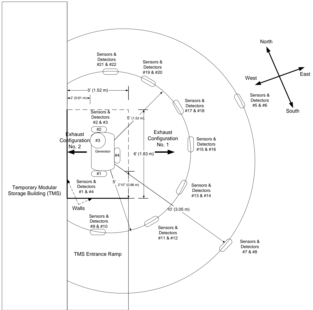
Figure 9: Plan View: Setup for Outdoor Tests Conducted under Two-Sided Roofed Shelter beside TMS.
