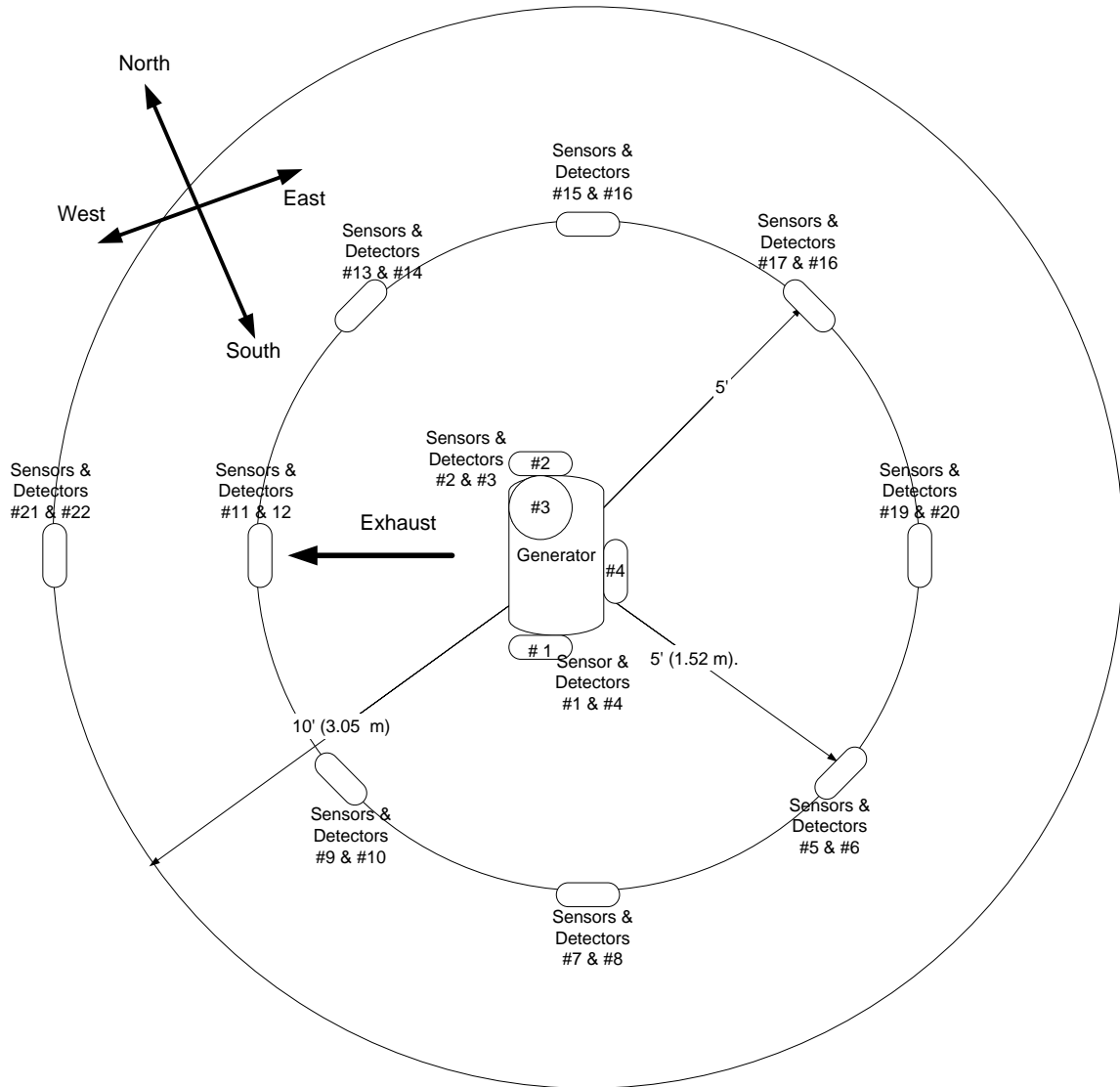
Figure 8: Plan View: Setup for Outdoor Tests Conducted in Center of Parking Area
