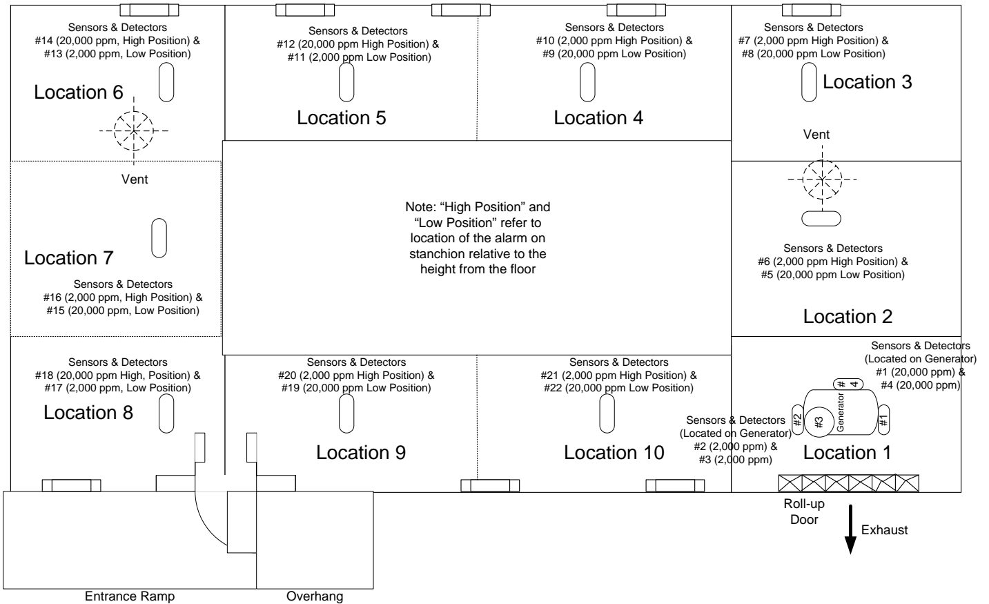
Figure 12: Plan View Inside TMS: Legend Showing Location of CO Sensors and CO Alarms and Where AER Calculations Were Performed
