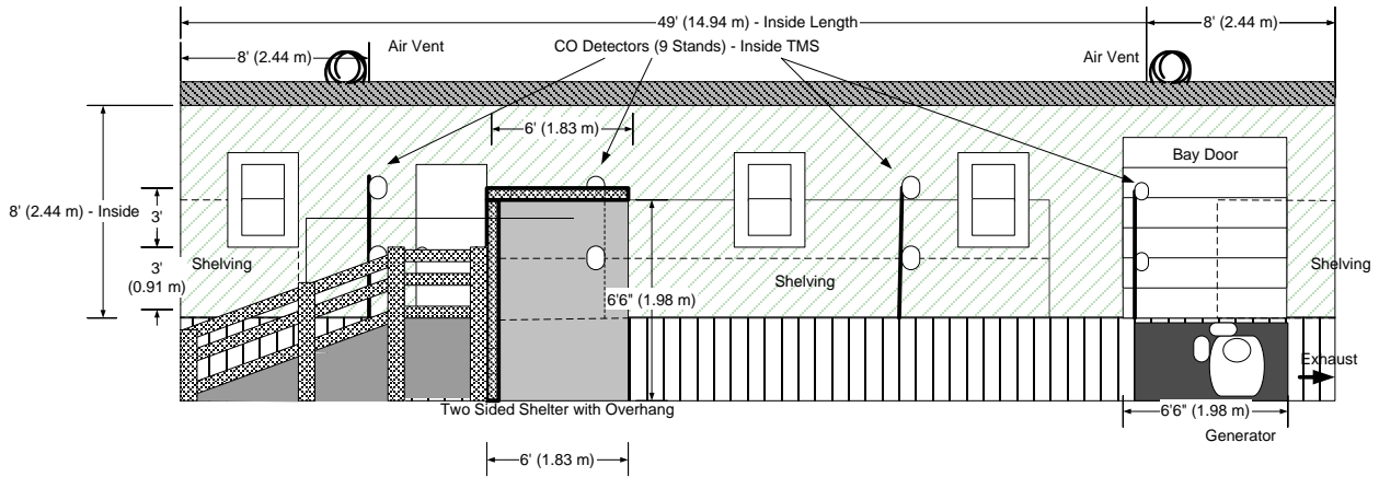
Figure 11: Elevation View: Setup for Tests Conducted Under TMS in Crawlspace
