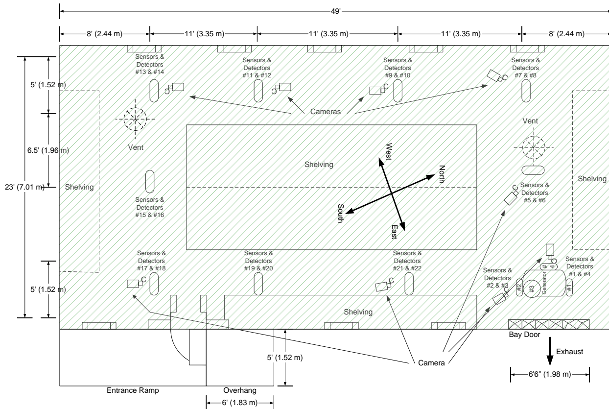
Figure 10: Plan View: Setup for Tests Conducted Inside TMS
